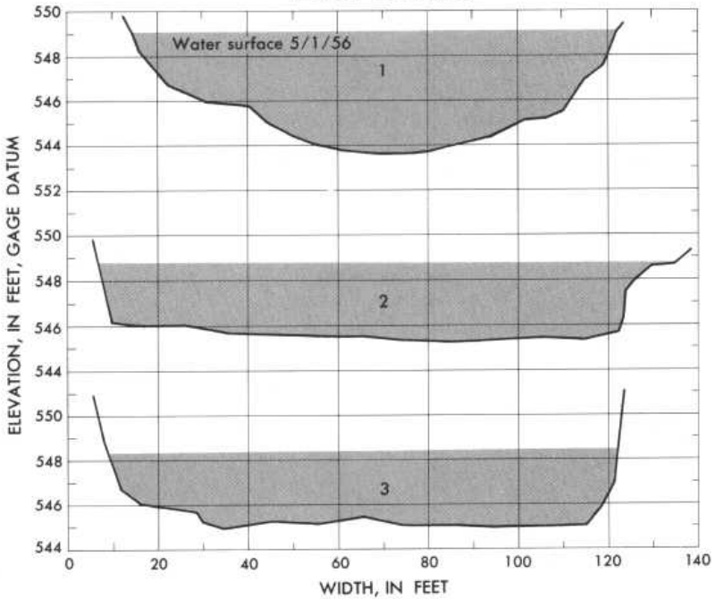
Plan sketch and cross sections, Middle Fork Vermilion River near Danville, Ill.
