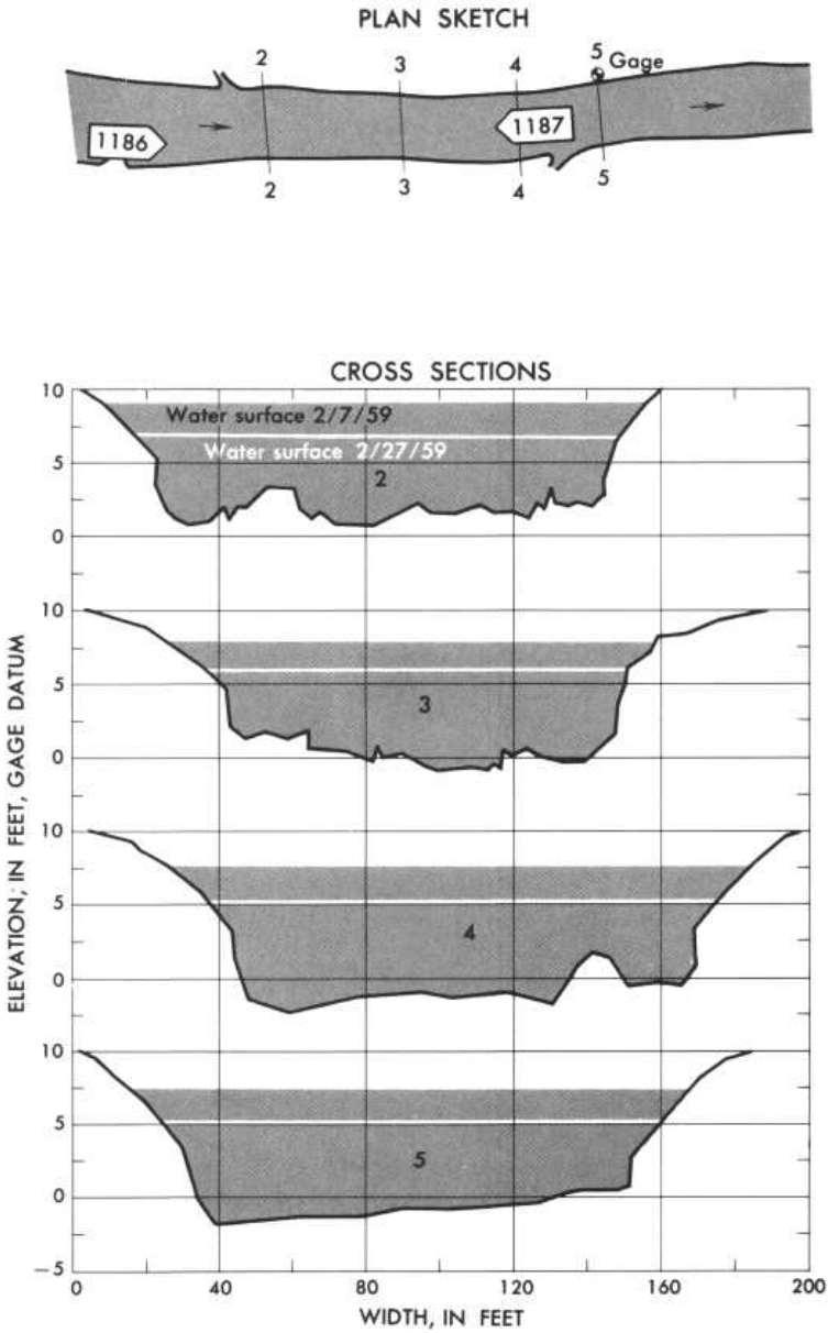
Plan sketch and cross sections, Chattahoochee River near Leaf, Ga.
