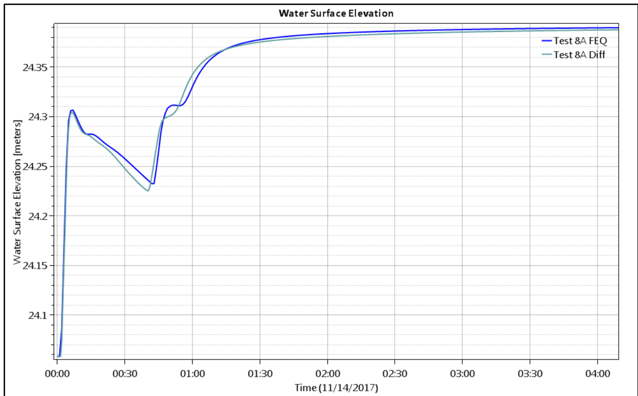
Figure 166. Test Point 5 - Water Level (depth) for Full Equations and Diffusion Wave.
