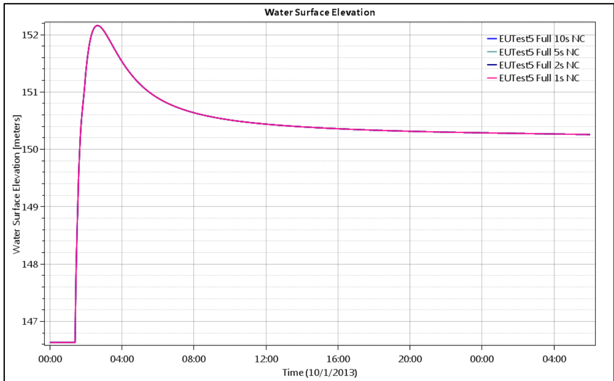
Figure 66. Test Point 4 - Water Level (depth), \Delta T = 1, 2, 5, 10 seconds.
