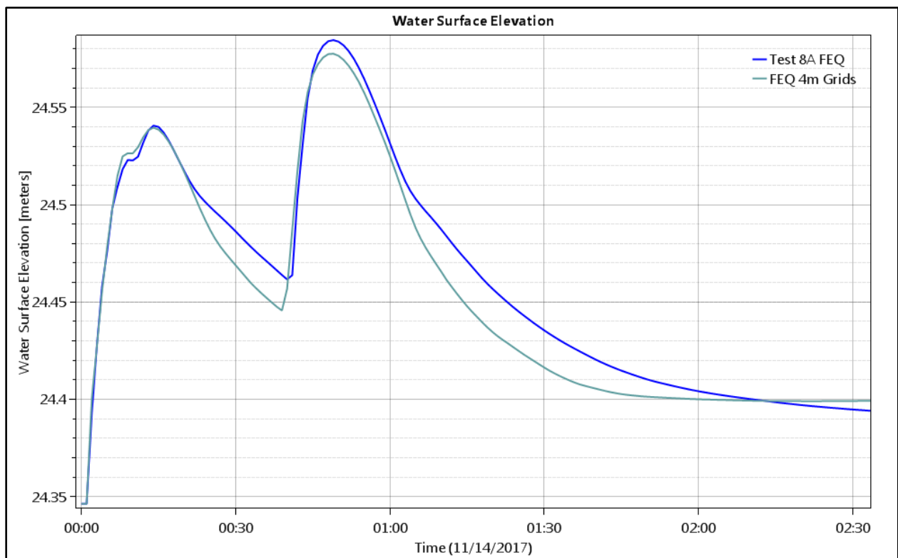
Figure 171. Test Point 4 - Water Level (depth) for Full Equations with 2m and 4m Grids.
