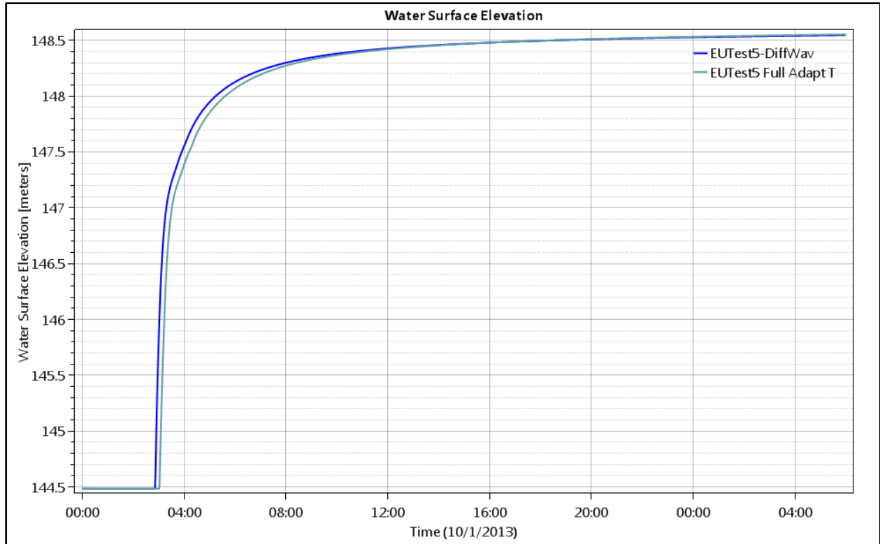
Figure 54. Test Point 5 - Water Level (depth) for Full Equations and Diffusion Wave.
