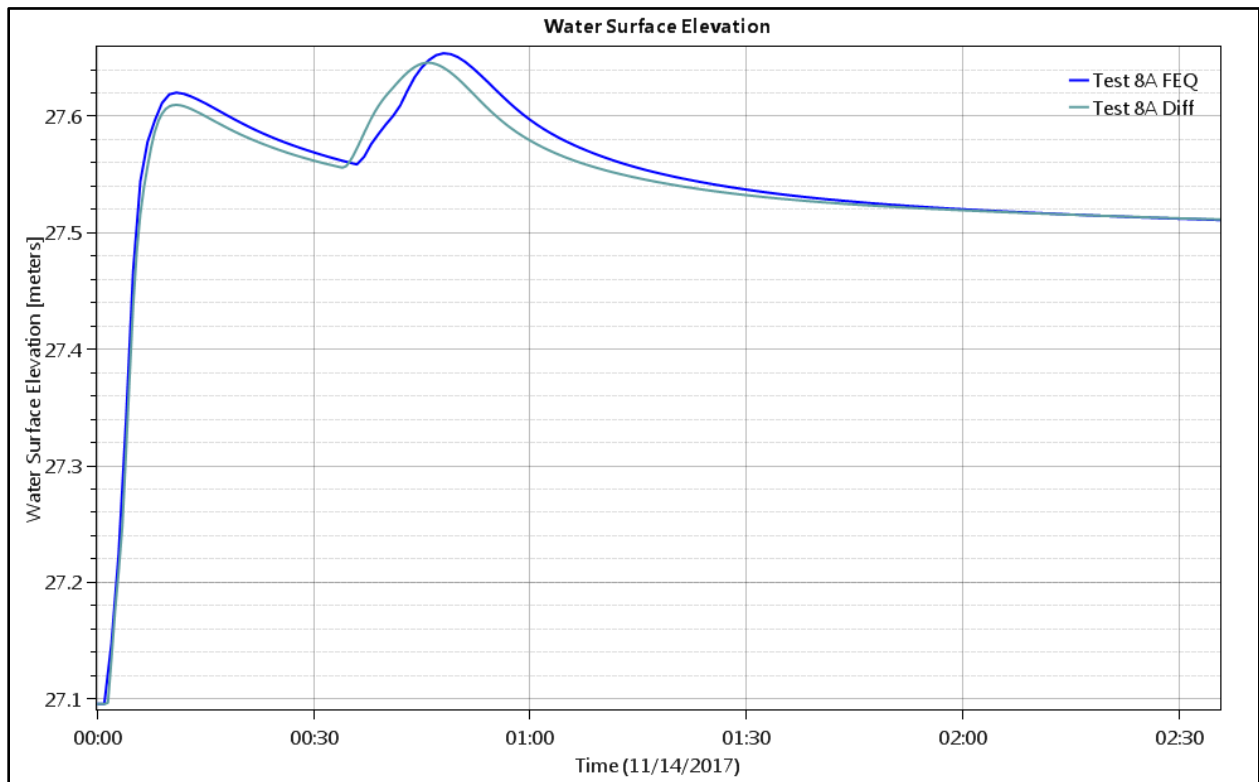
Figure 162. Test Point 1 - Water Level (depth) for Full Equations and Diffusion Wave.
