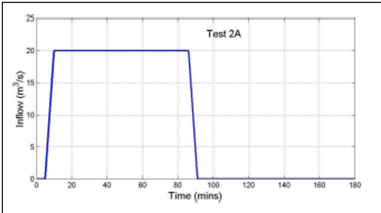
Figure 6. Inflow hydrograph used as upstream boundary condition.
