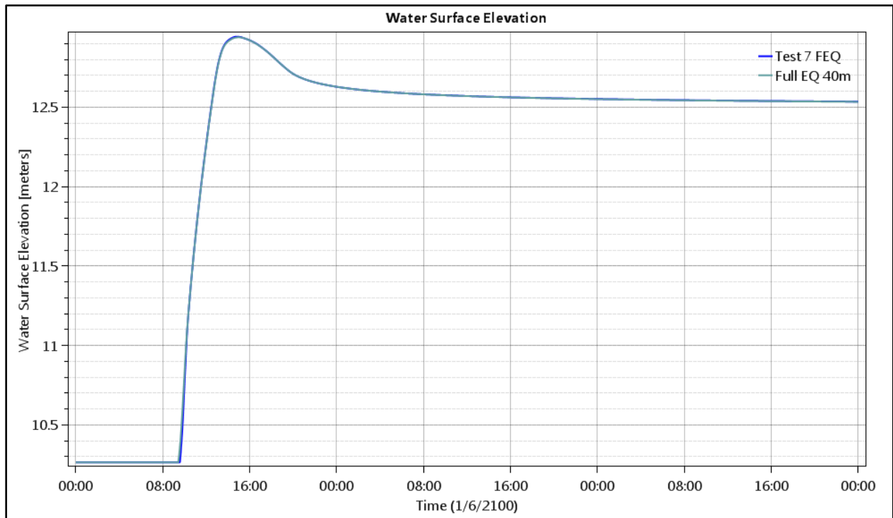
Figure 151. Floodplain 2 - Test Point 8 - Water Level.
