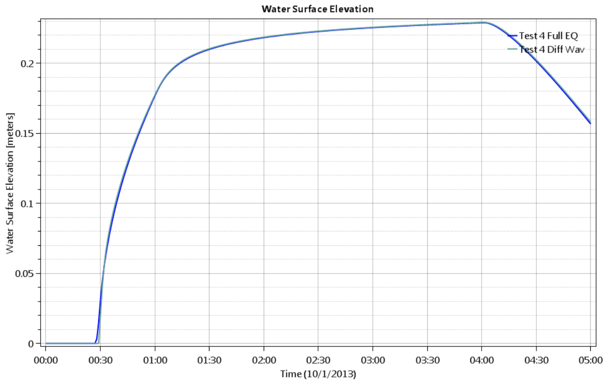
Figure 30. Test Point 3 Water Level (depth).
