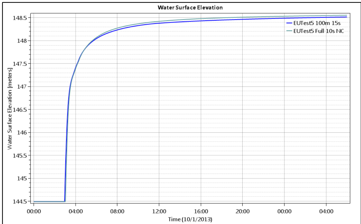
Figure 78. Test Point 5 - Water Level (depth), 50 and 100 meter grids.
