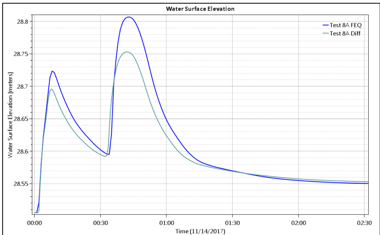
Figure 163. Test Point 2 - Water Level (depth) for Full Equations and Diffusion Wave.
