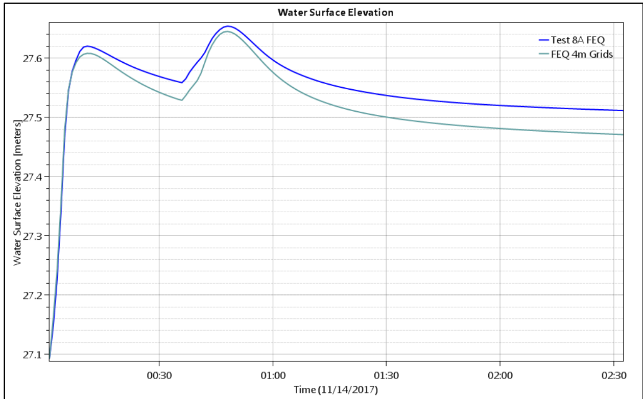
Figure 168. Test Point 1 - Water Level (depth) for Full Equations with 2m and 4m Grids.
