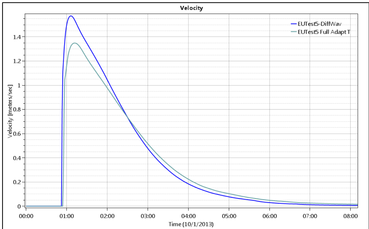
Figure 59. Test Point 7 - Velocity Time Series for Full Equations and Diffusion Wave.
