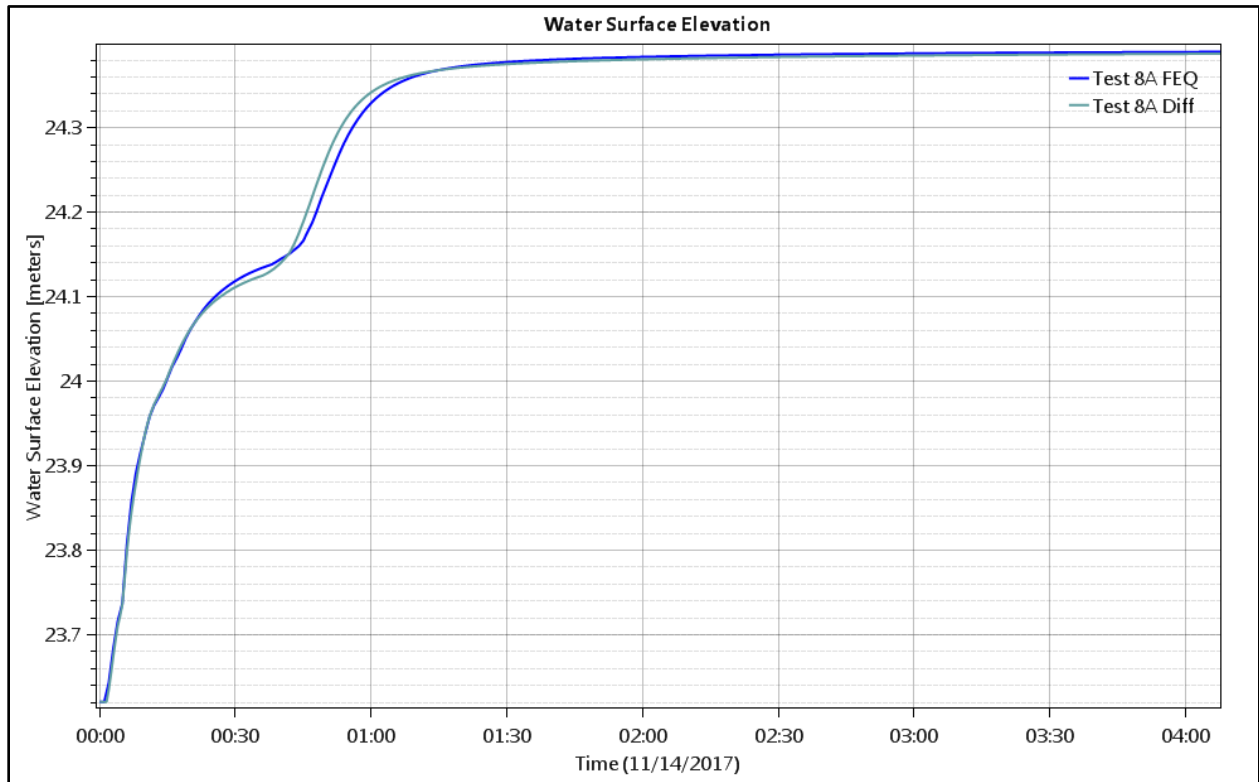
Figure 164. Test Point 3 - Water Level (depth) for Full Equations and Diffusion Wave.
