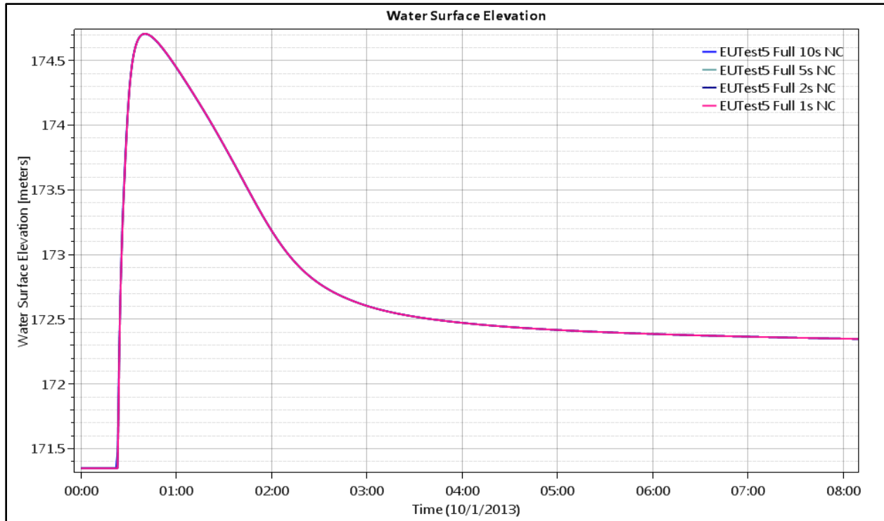
Figure 60. Test Point 1 - Water Level (depth), \Delta T = 1, 2, 5, 10 seconds.
