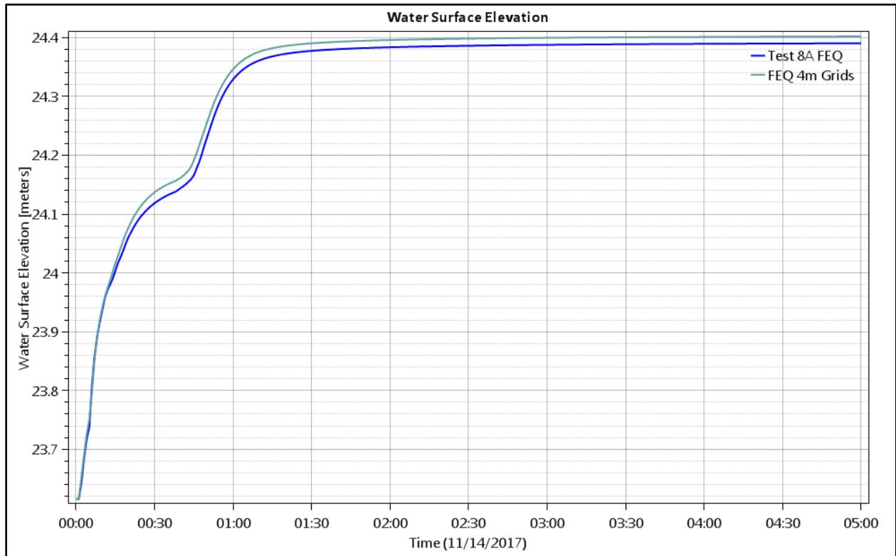
Figure 170. Test Point 3 - Water Level (depth) for Full Equations with 2m and 4m Grids.
