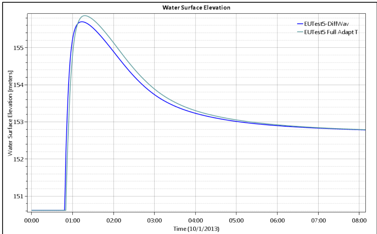
Figure 50. Test Point 3 - Water Level (depth) for Full Equations and Diffusion Wave.
