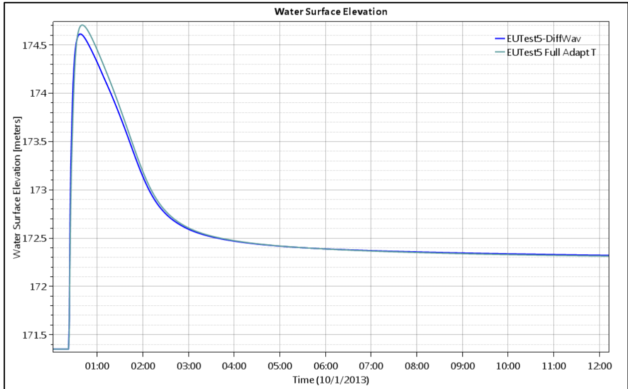
Figure 46. Test Point 1 - Water Level (depth) for Full Equations and Diffusion Wave.
