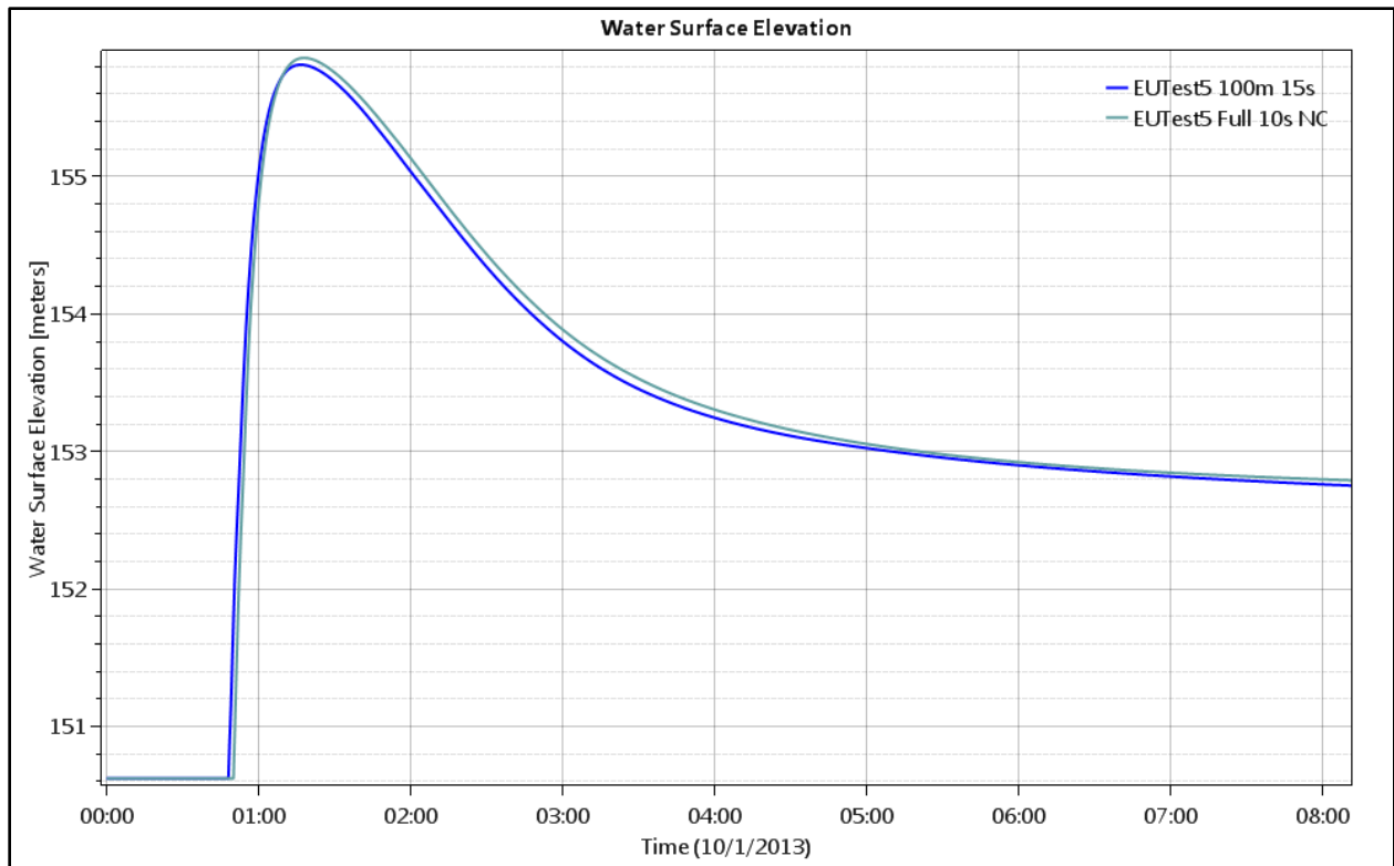
Figure 74. Test Point 3 - Water Level (depth), 50 and 100 meter grids.
