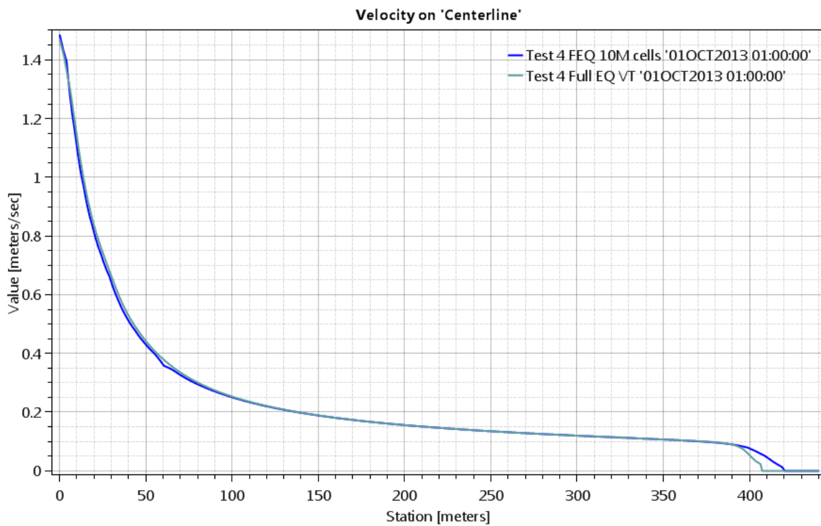
Figure 43. Velocity versus Distance at Time 1HOUR.
