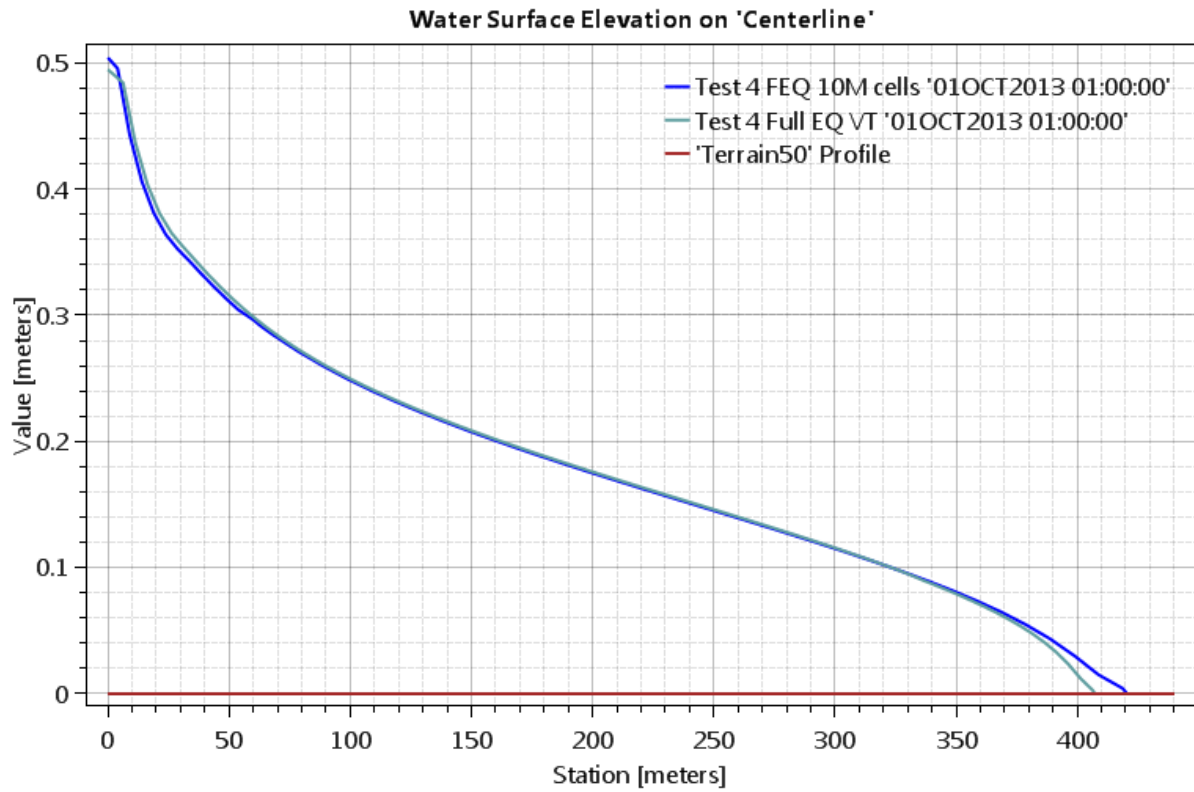
Figure 42. Depth versus Distance at Time 1HOUR.
