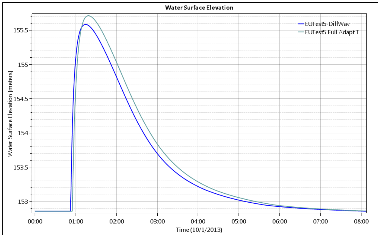
Figure 58. Test Point 7 - Water Level (depth) for Full Equations and Diffusion Wave.
