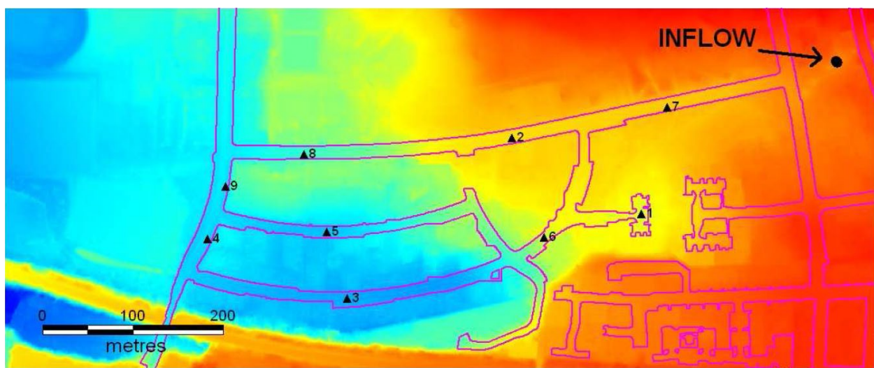
Figure 159. DEM for Test 8A.
