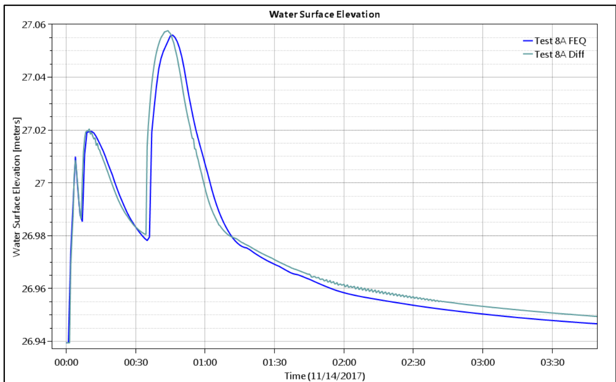
Figure 167. Test Point 6 - Water Level (depth) for Full Equations and Diffusion Wave.
