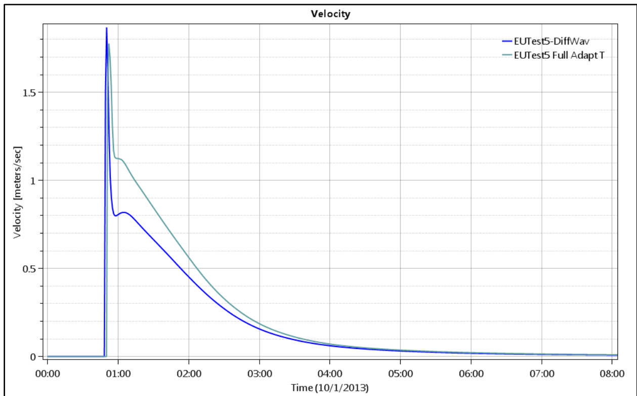
Figure 51. Test Point 3 - Velocity Time Series for Full Equations and Diffusion Wave.
