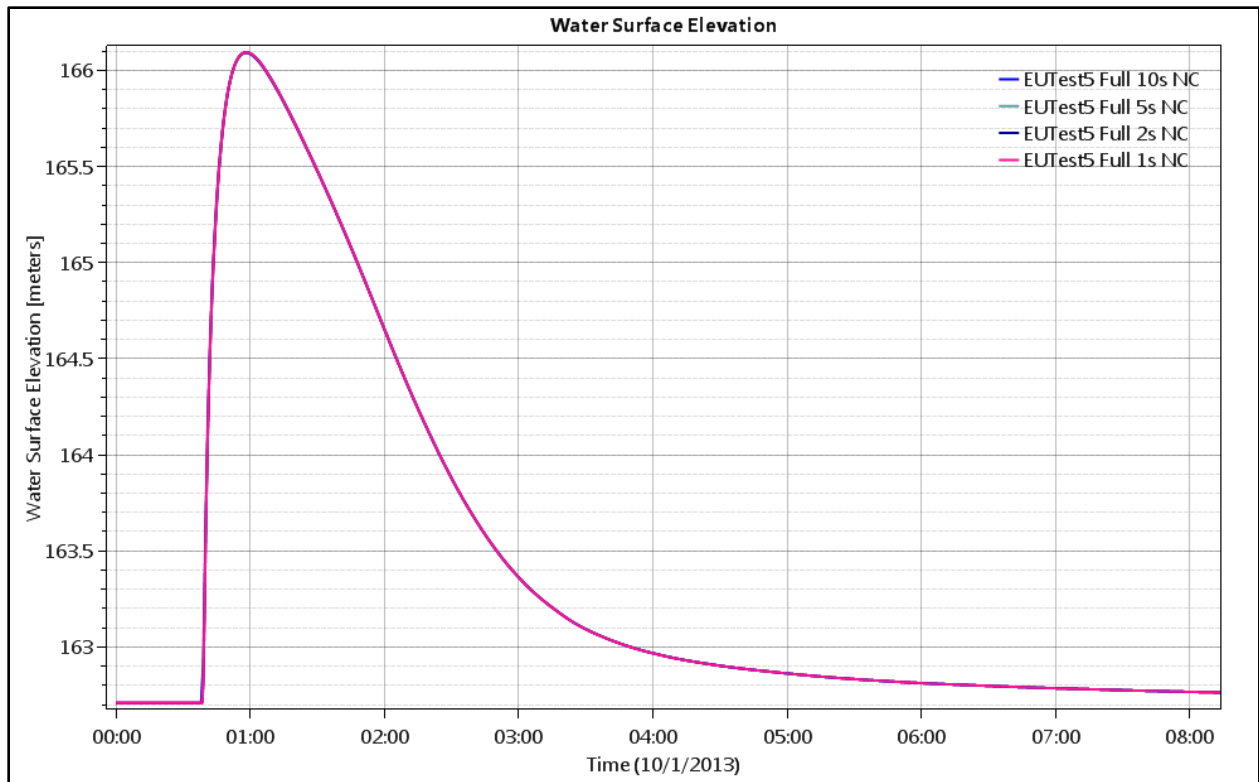
Figure 62. Test Point 2 - Water Level (depth), \Delta T = 1, 2, 5, 10 seconds.
