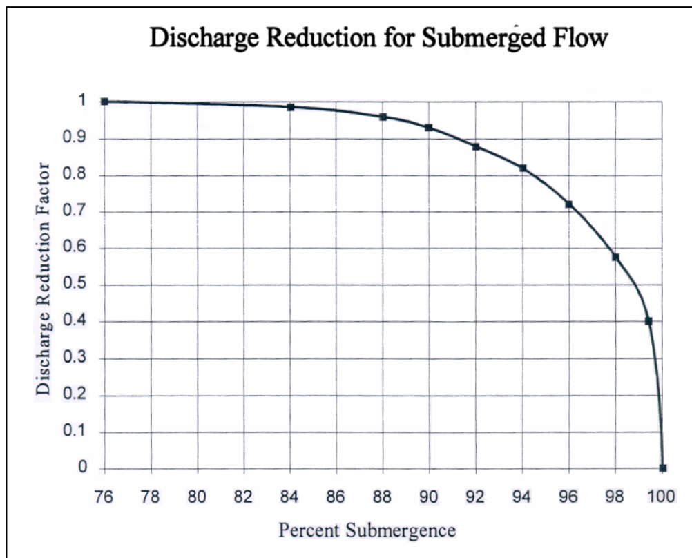
Figure 7. Factor for reducing weir flow for submergence
