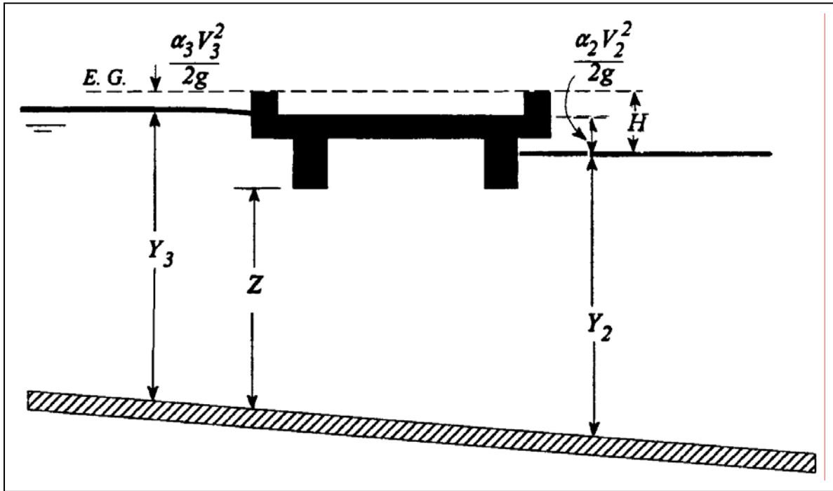
Figure 5. Example of a bridge under fully submerged pressure flow
