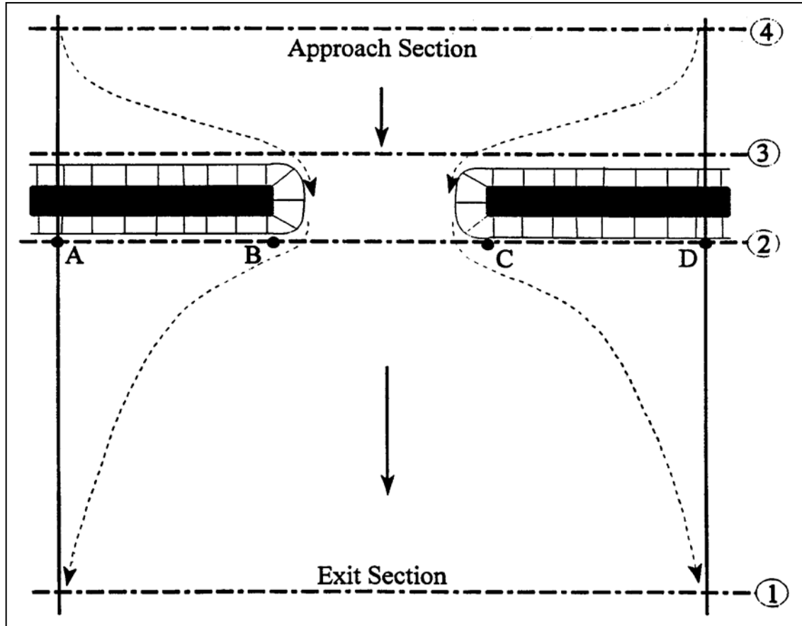
Figure 1. HEC-RAS Cross Section Locations at a Bridge
