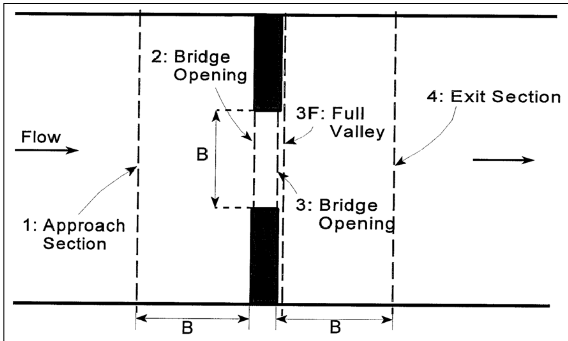
Figure 8. Cross section locations for WSPRO bridge hydraulics
