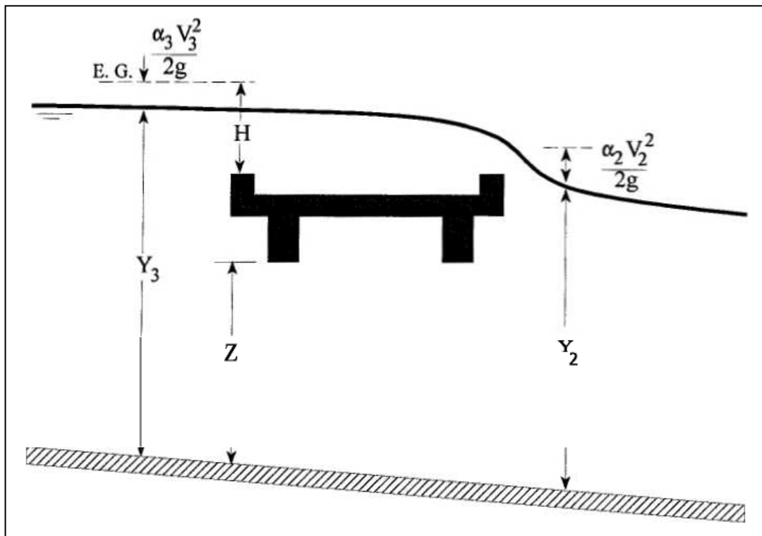
Figure 6. Example bridge with pressure and weir flow
