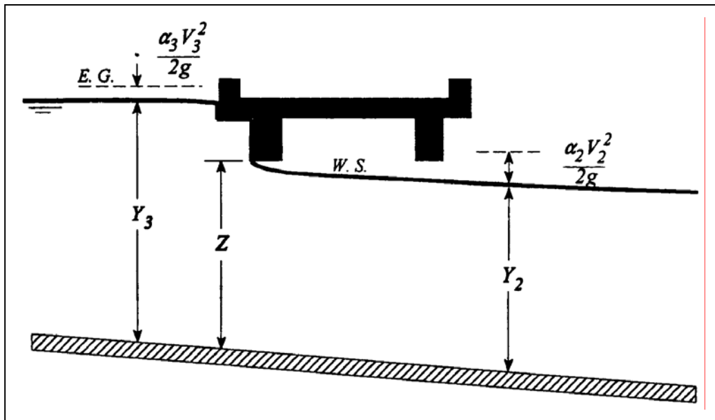
Figure 3. Example of a bridge under sluice gate type of pressure flow
