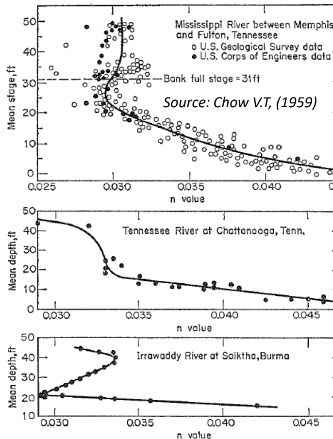
FIG. 5-4. Variations of the n value with the mean stage or d
