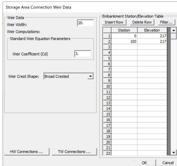
Figure 2. Storage Area Connection Weir Data editor.
