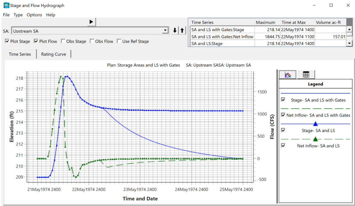
Figure 11. Upstream Storage Area.
