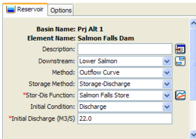
Figure 131. Reservoir component editor using the outflow curve routing method with a storage-discharge function.
