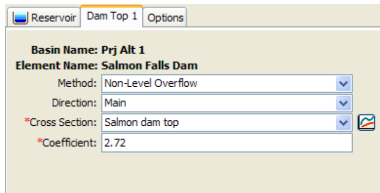
Figure 142. Dam top editor with the non-level overflow method selected.
