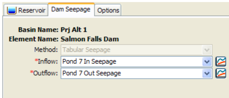
Figure 146. Dam seepage editor showing seepage into a reservoir.
