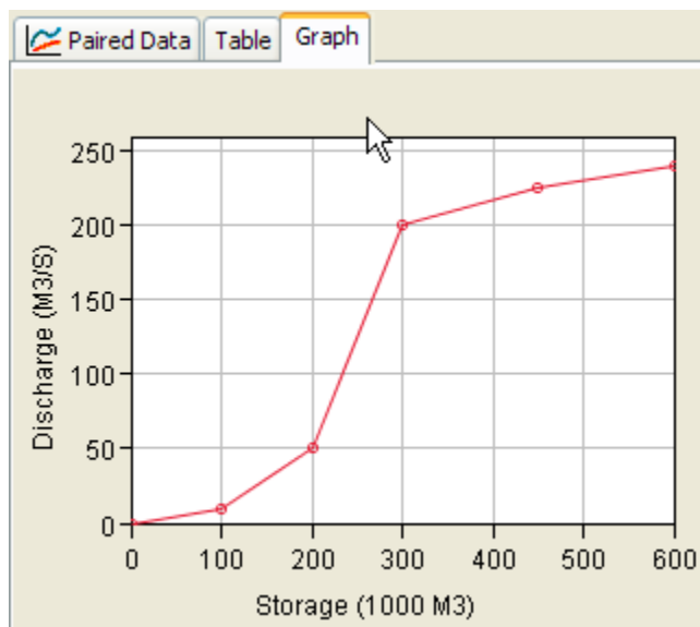
Figure 60. Viewing data for a storage-discharge curve.
