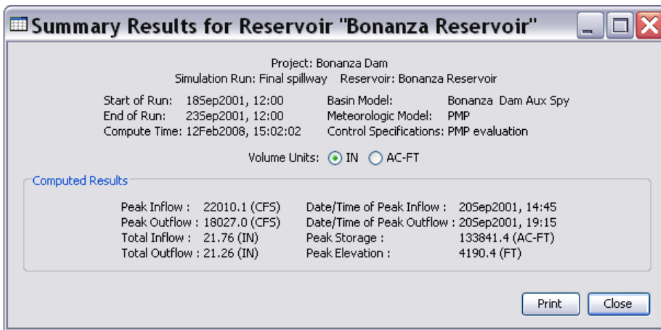
14 Summary Results for Bonanza Reservoir
