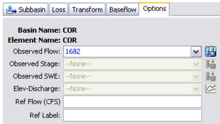
1 Adding Observed Flow for Calibration
