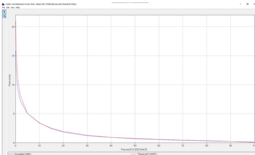
33 Flow Duration Curves for HMS and HSPF
