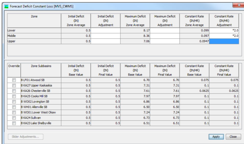
16 Forecast Deficit and Constant Loss Parameter Adjustment Editor
