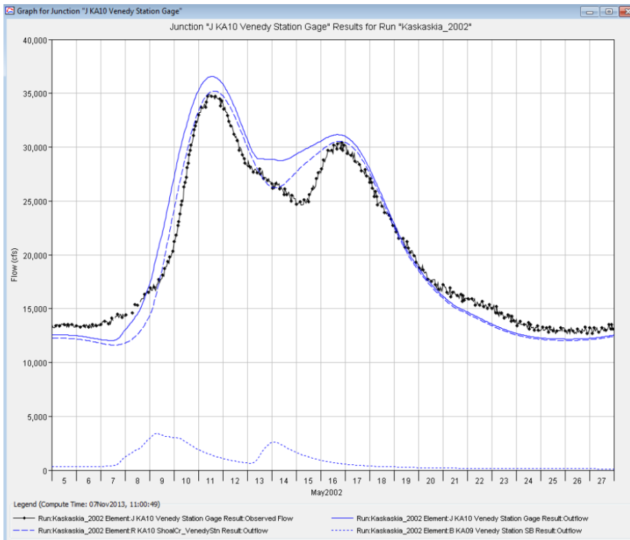
17 2002 Wet/Typical Calibrated Hydrographs at the Venedy Gage
