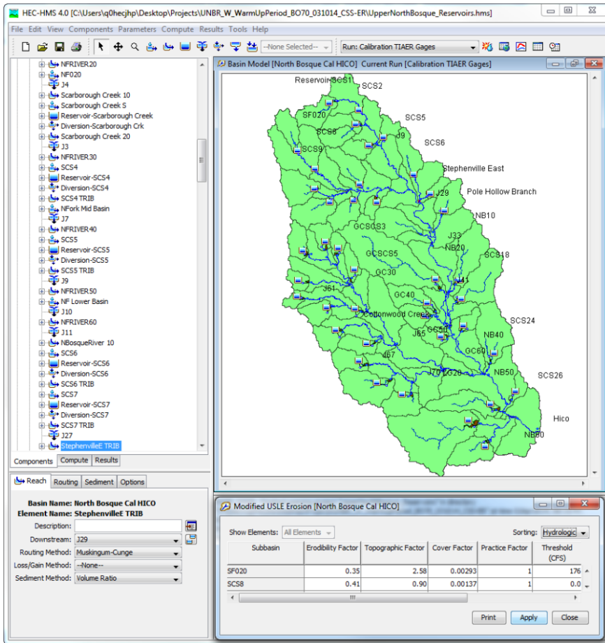
15 Sediment Model Setup in HEC-HMS
