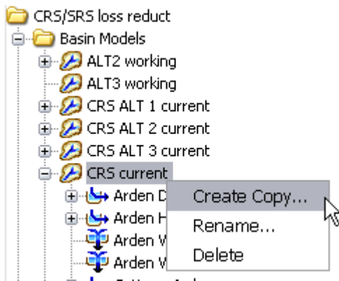
10 Copying a Basin Model
