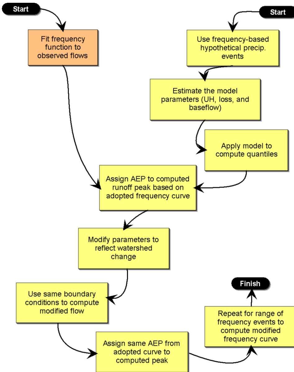
5 Method 2 Steps to Calibrate Models to Flow-Frequency Function
