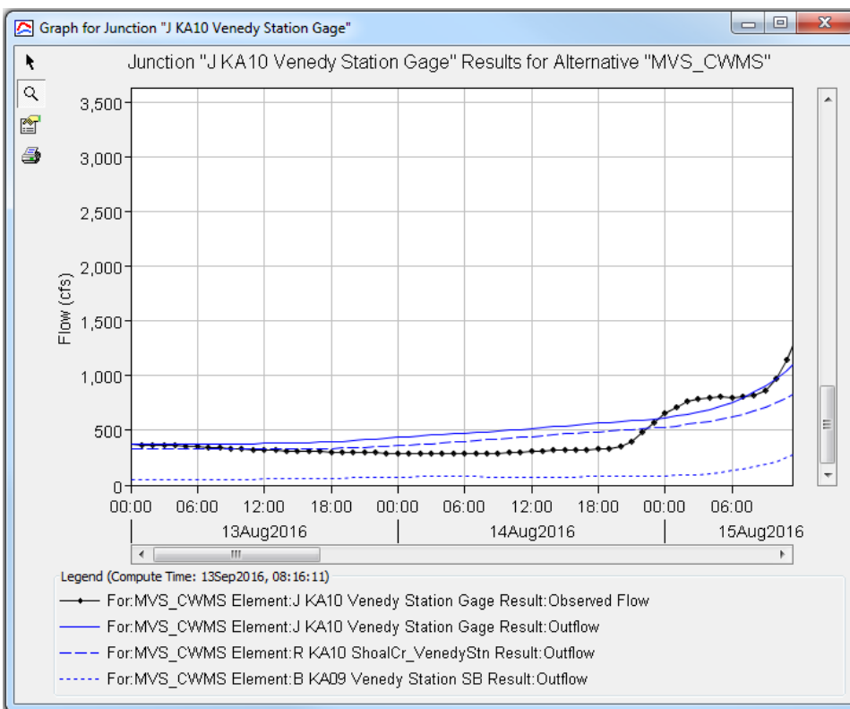
22 Initial Baseflow at the Venedy Station Gage
