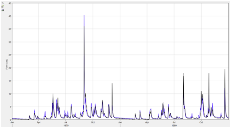
31 Comparison between HEC-HMS and HSPF daily hydrographs
