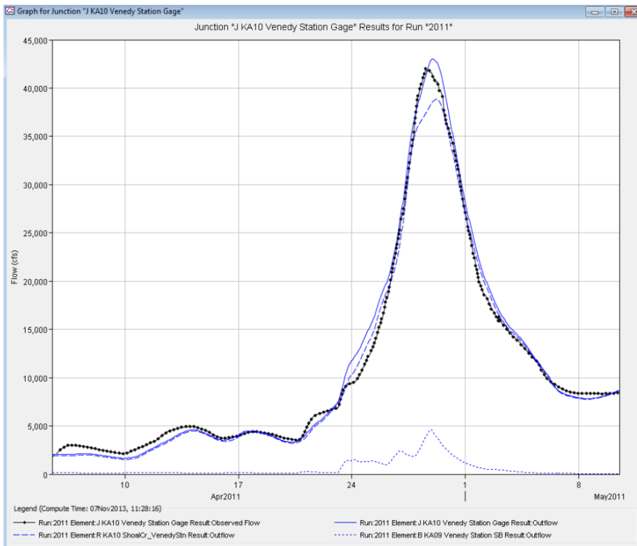
19 2011 Wet/Typical Calibrated Hydrographs at the Venedy Gage
