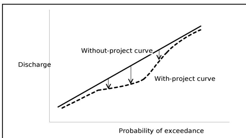
7 Conceptual Effect of Alternative 1 on the Flow-Frequency Curve
