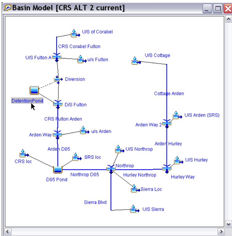
8 Basin Model for Alternative 2
