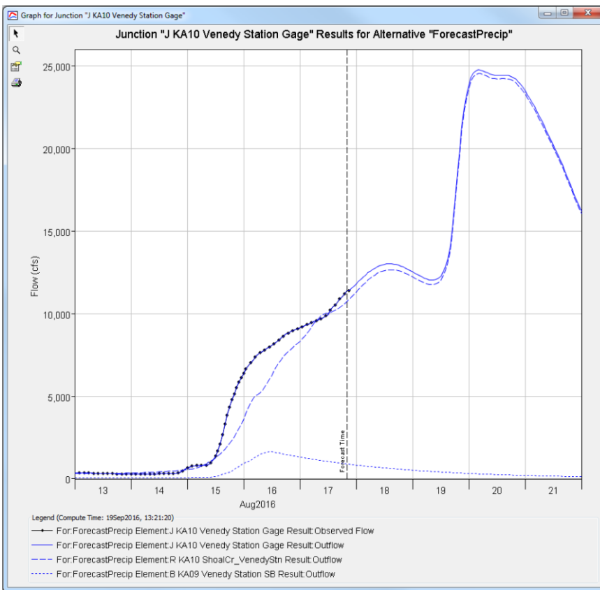
26 Venedy Station Gage Results Assuming Forecasted Precipitation
