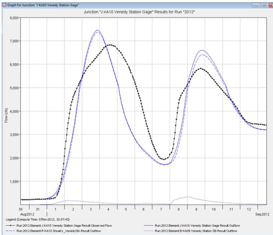
20 2012 Dry Calibrated Hydrographs at the Venedy gage
