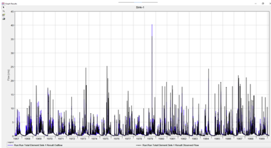
32 HEC-HMS runoff time series vs HSPF's runoff time series
