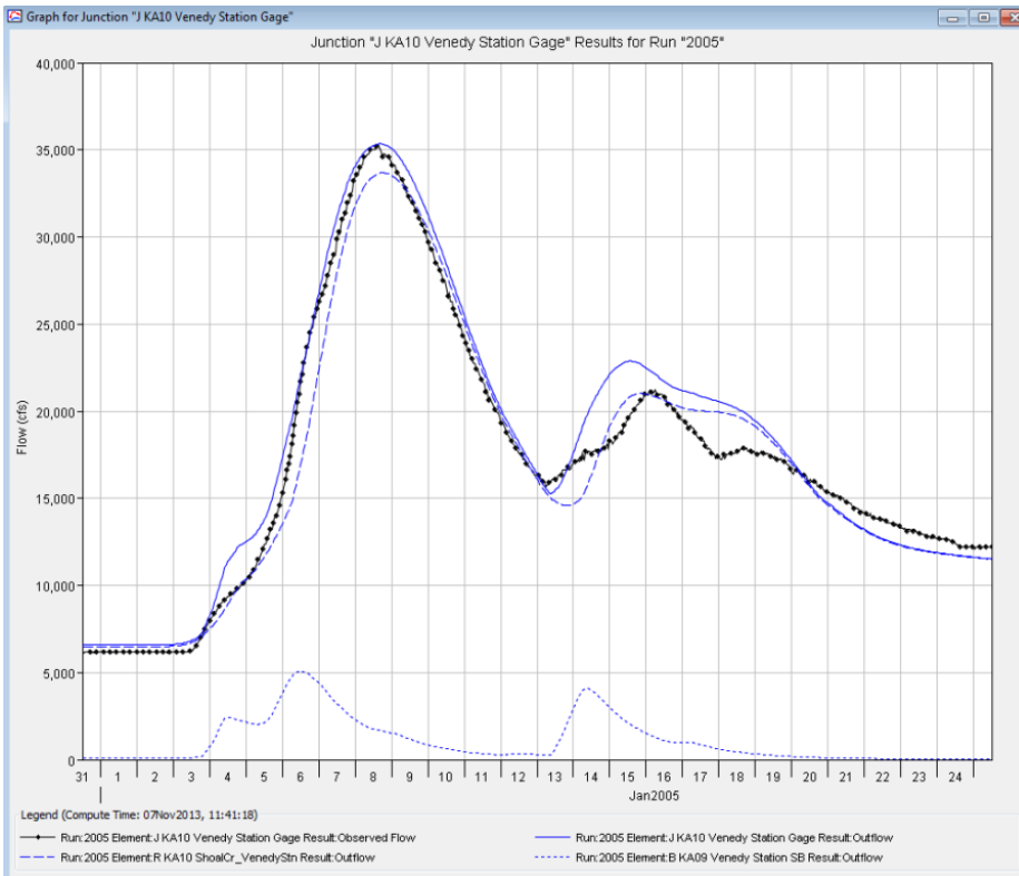
18 2005 Wet/Snowmelt Calibrated Hydrographs at the Venedy Gage
