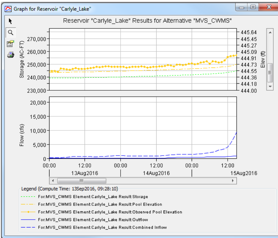
24 Carlyle Lake Reservoir Initialization
