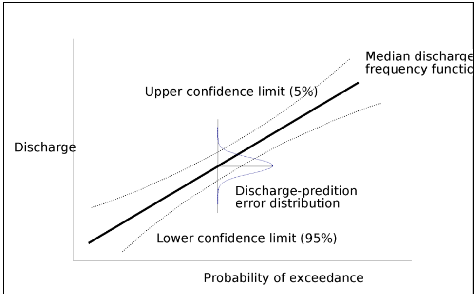
11 Flow-Frequency Function with Uncertainty Distribution
