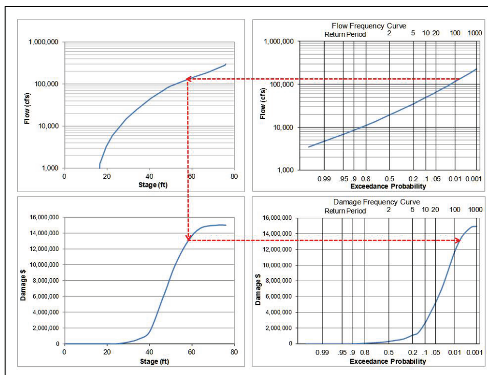
Figure G.12 Transformation from Flow-Frequency Curve to Damage-Frequency Curve in CDF (cumulative) Form
