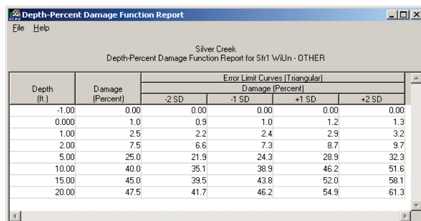
Figure 9.10 Depth-Percent Damage Function Report - Other Dialog Box
