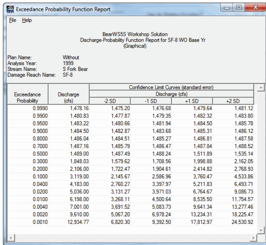
Figure 5.7 Exceedance Probability Function Report - Graphical - From Water Surface Profiles - Eight Data Points
