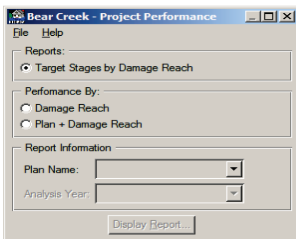
Figure 15.8 Project Performance Dialog Box
