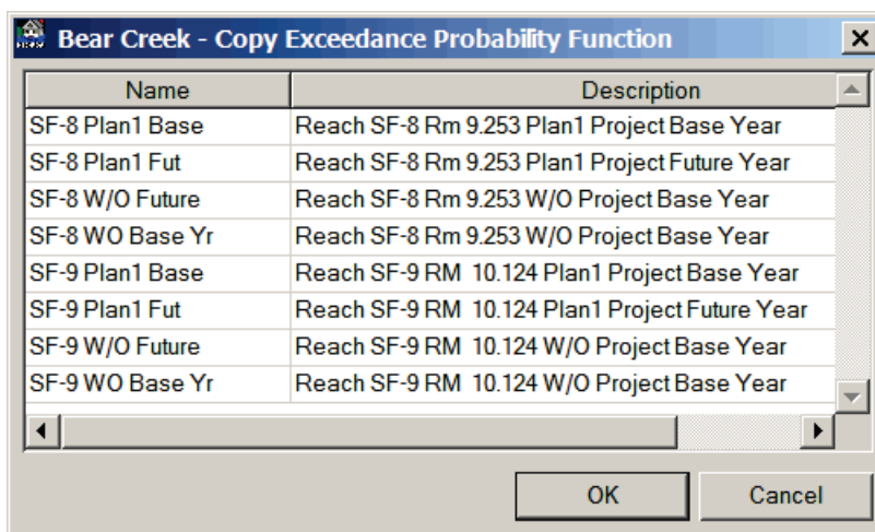
Figure 5.16 Copy Exceedance Probability Function Dialog Box
