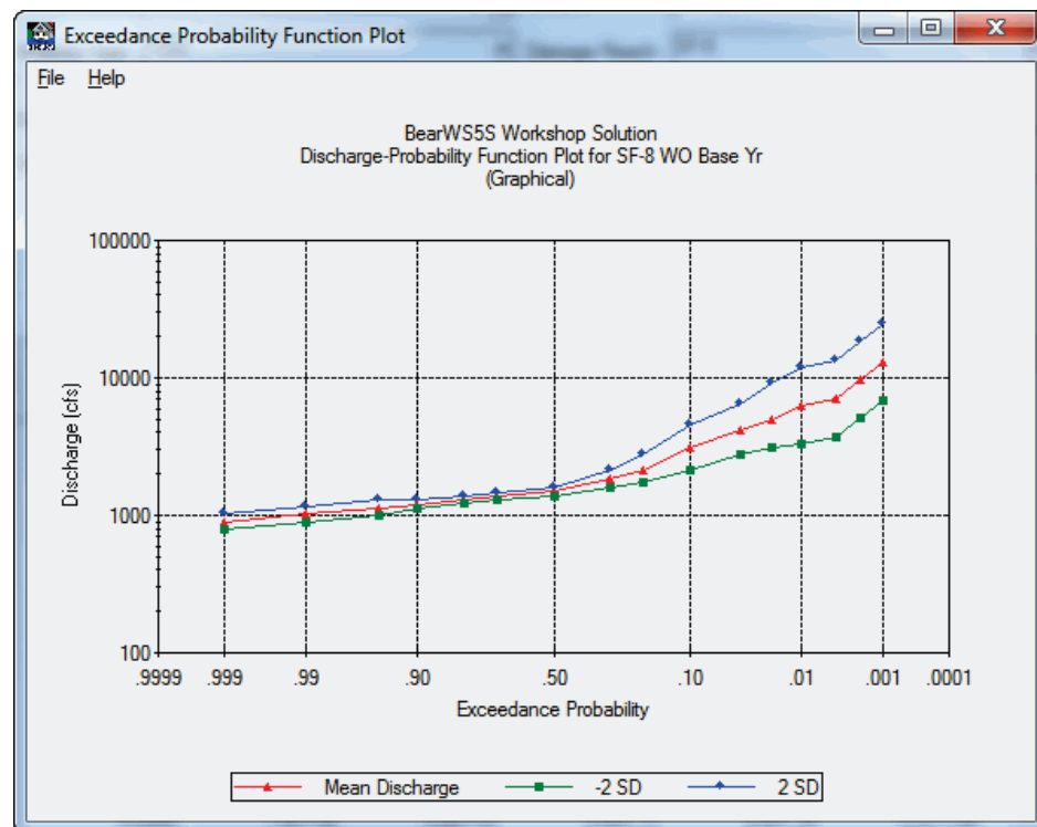
Figure 5.10 Exceedance Probability Function Plot - Graphical - Nine Data Points
