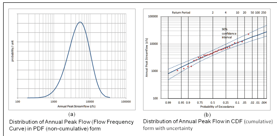
Figure G.11 Distribution of Annual Peak Flow
