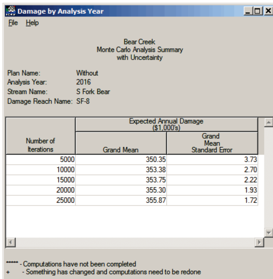
Figure 14.6 Monte Carlo Analysis Summary with Uncertainty -Report
