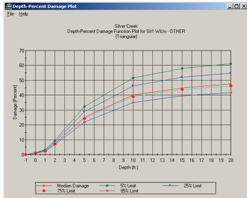
Figure 9.9 Depth-Percent Damage Function Plot - Other Dialog Box
