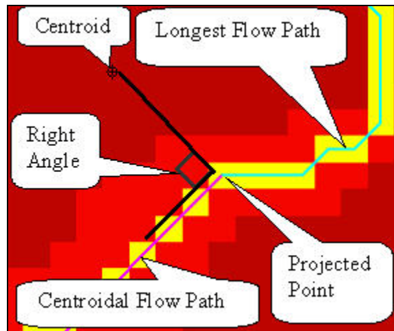
Figure 9-13. Centroidal Flow Path.
