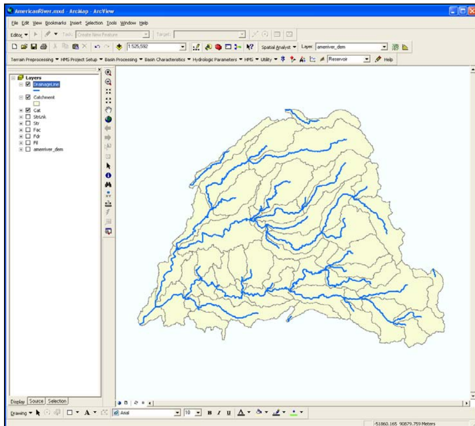
Figure 13-15. Drainage Lines.
