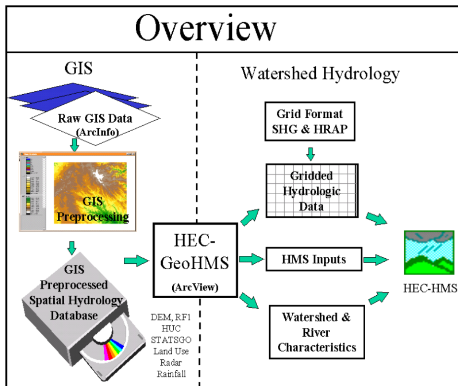
Figure 3-1. Overview of GIS and Hydrology Programs.
