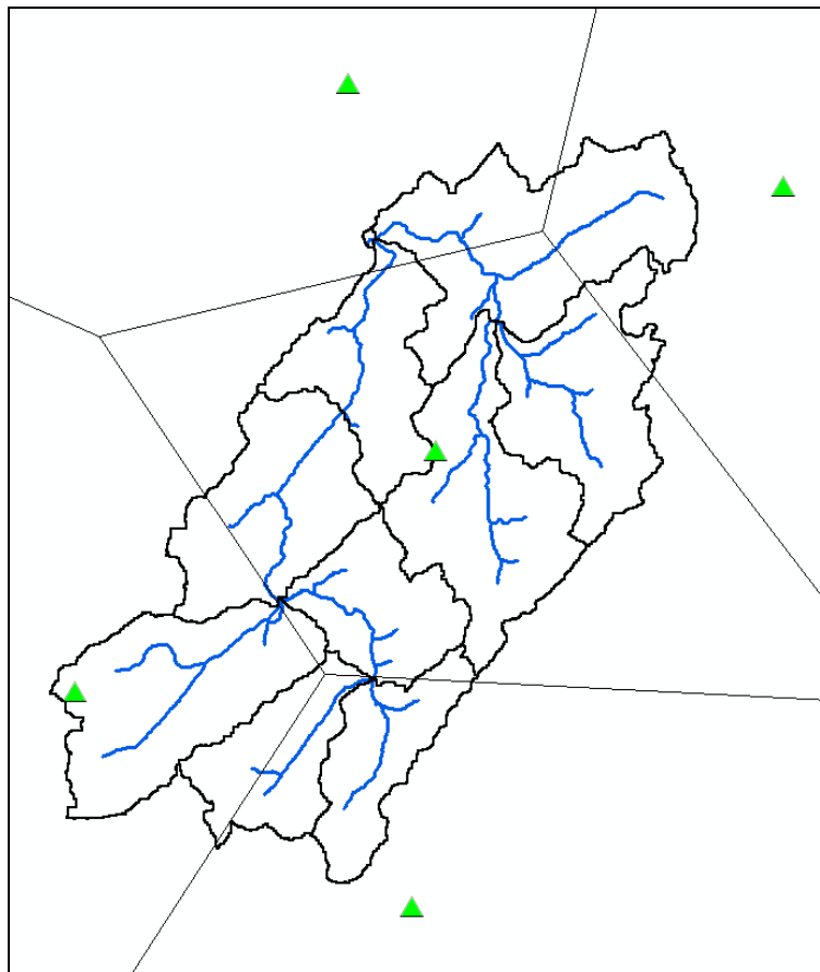
Figure 11-20. Thiessen Polygons.
