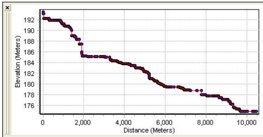
Figure 8-12. River Profile.
