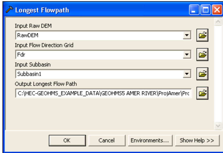
Figure 13-35. Longest Flow Path Computation Editor.
