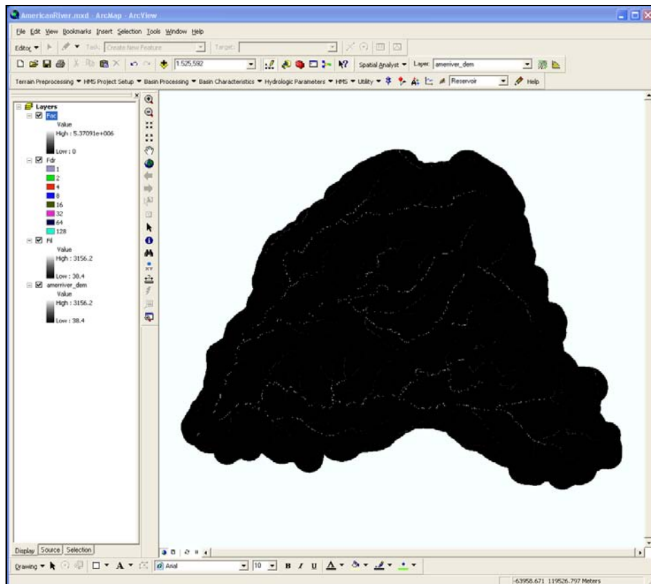
Figure 13-8. Flow Accumulation Grid.
