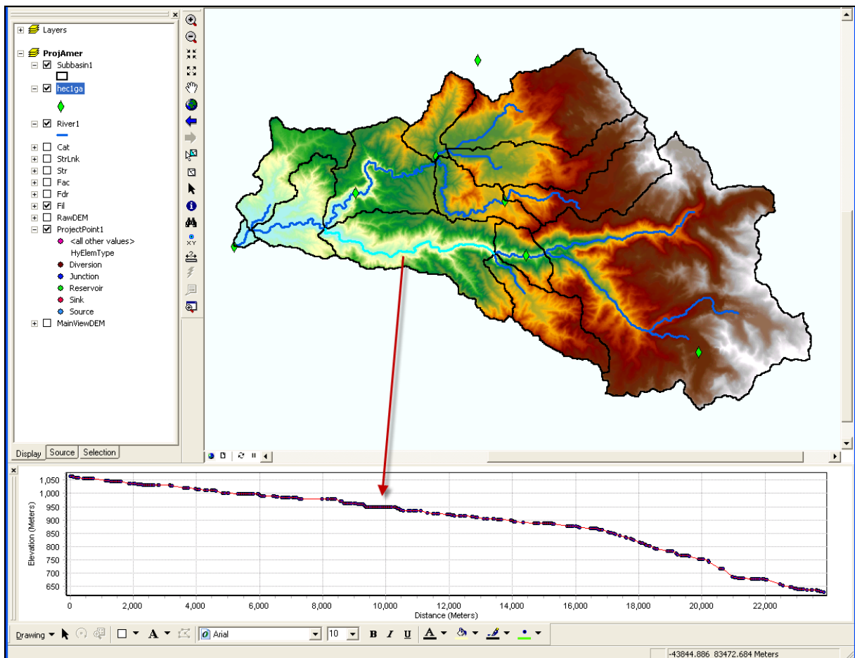
Figure 13-32. Profile for Selected Reach.
