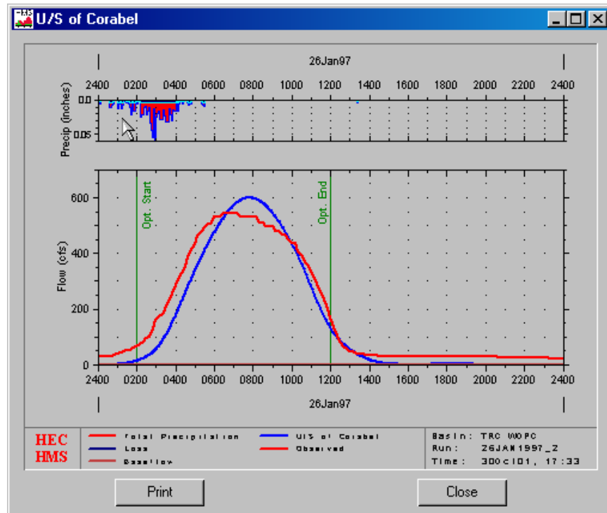
Figure 7. Verification of estimated parameters with January 26, 1997 event
