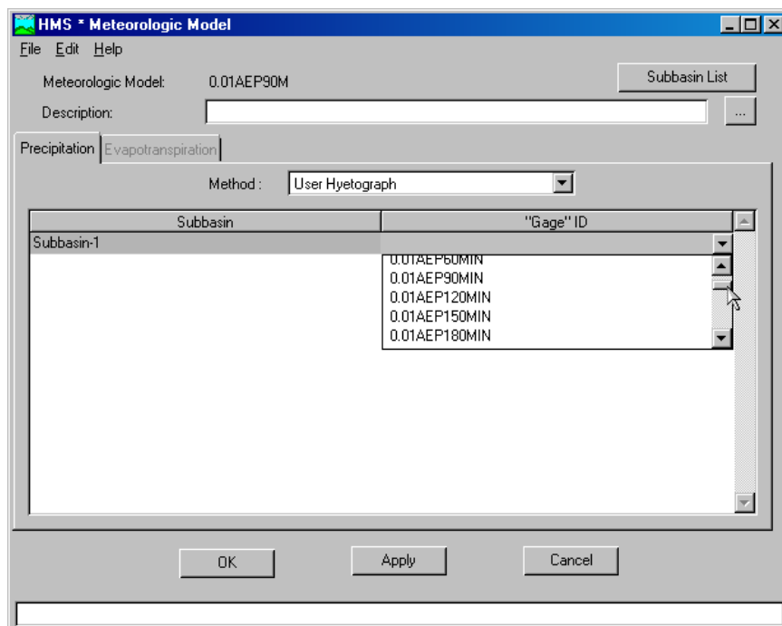
Figure 39. User hyetograph is selected and gage identified with Meteorologic Model form
