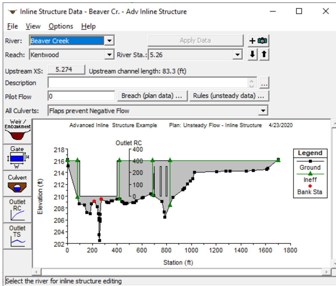
Figure 18-2. Inline Structure Data Editor
