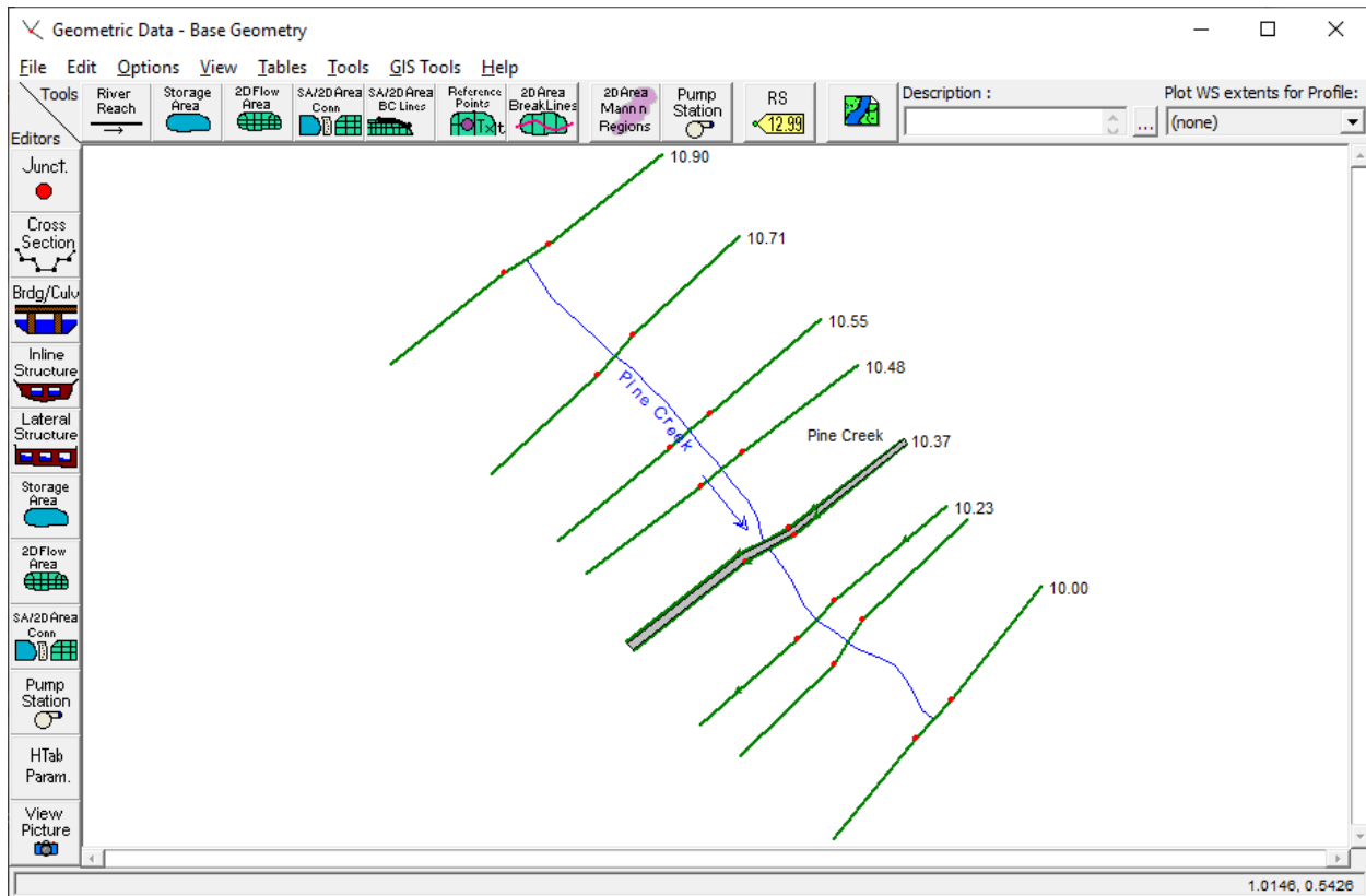
Figure 11-1: River System Schematic
