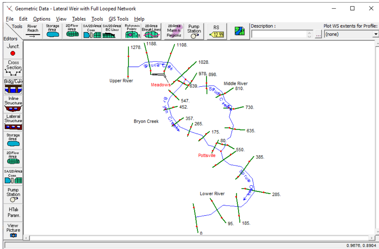
Figure 15-1: River System Schematic for Split Flow Example
