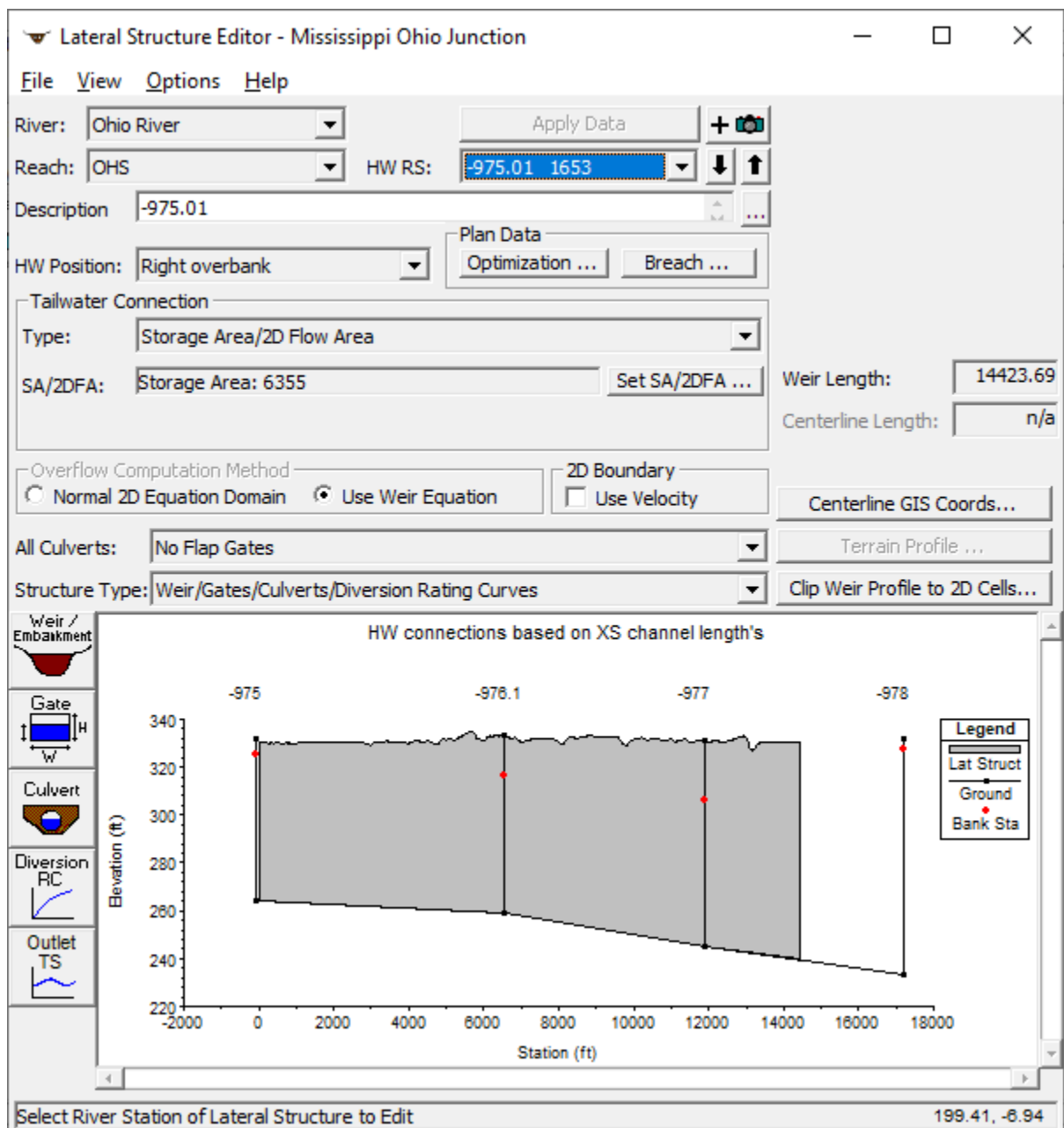
Figure 24-6. Lateral Weir Data Editor
