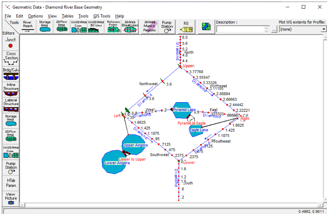
Figure 17-1: River System Schematic for Diamond River Base Geometry
