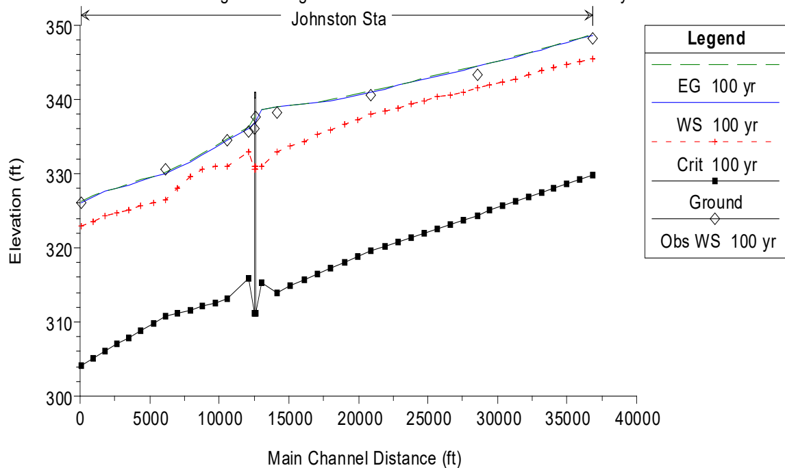
Figure 13-16: Water Surface Profile #2 for Bogue Chitto
