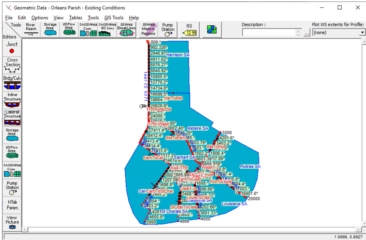
Figure 23-1. River System Schematic for New Orleans Parish System shown within the Geometric Data Editor
