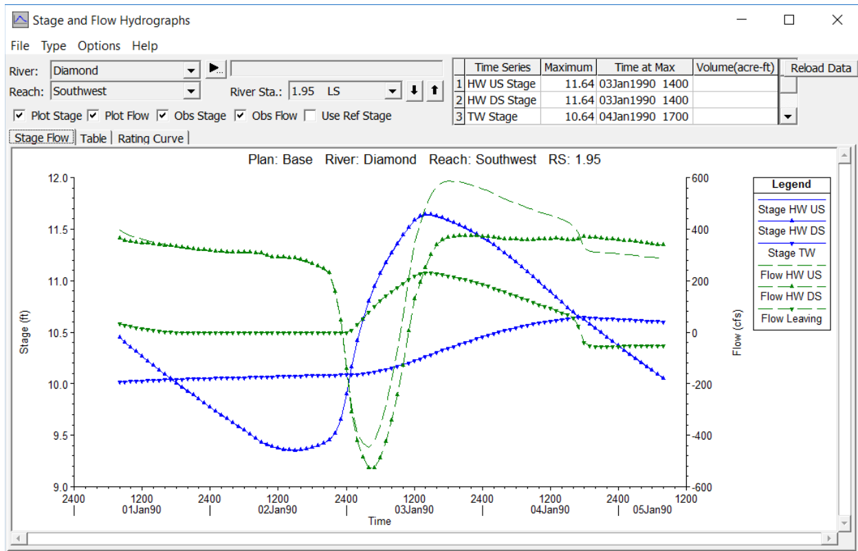
Figure 17-23: Stage and Flow Hydrograph for Lateral Structure Located on the Southwest Reach
