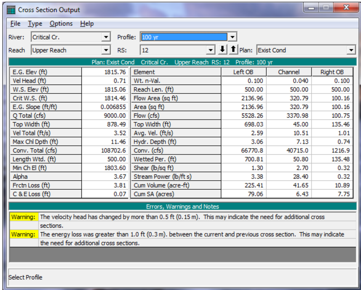
Figure 1-6: Cross Section Table For River Station 12
