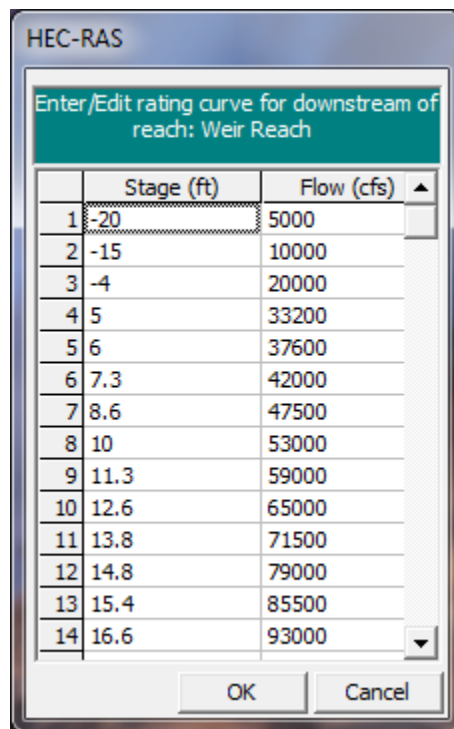
Figure 12-10: Rating Curve Editor
