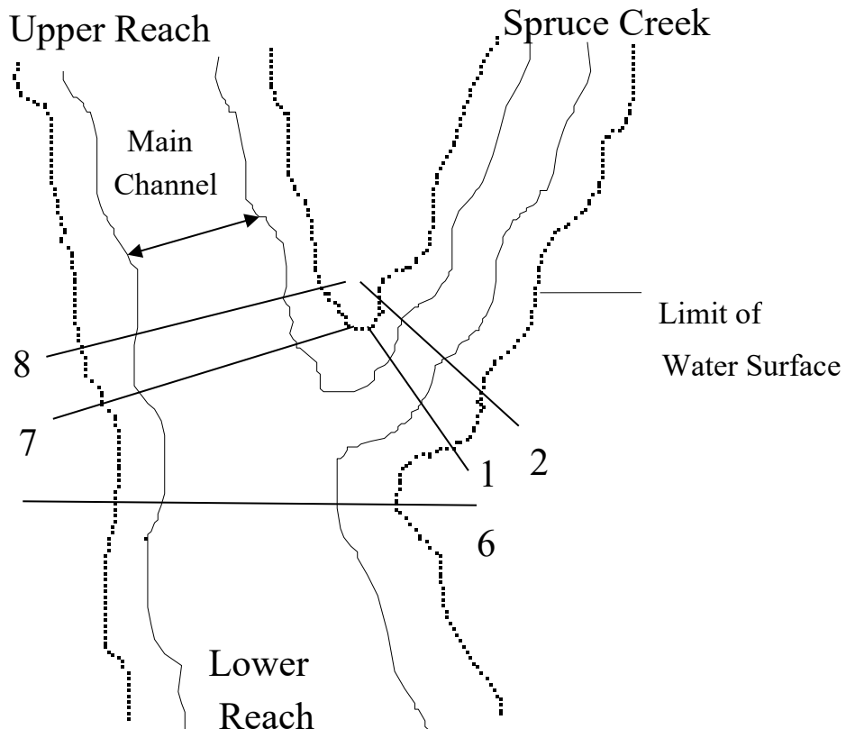
Figure 10-2: Cross Section Placement Schematic
