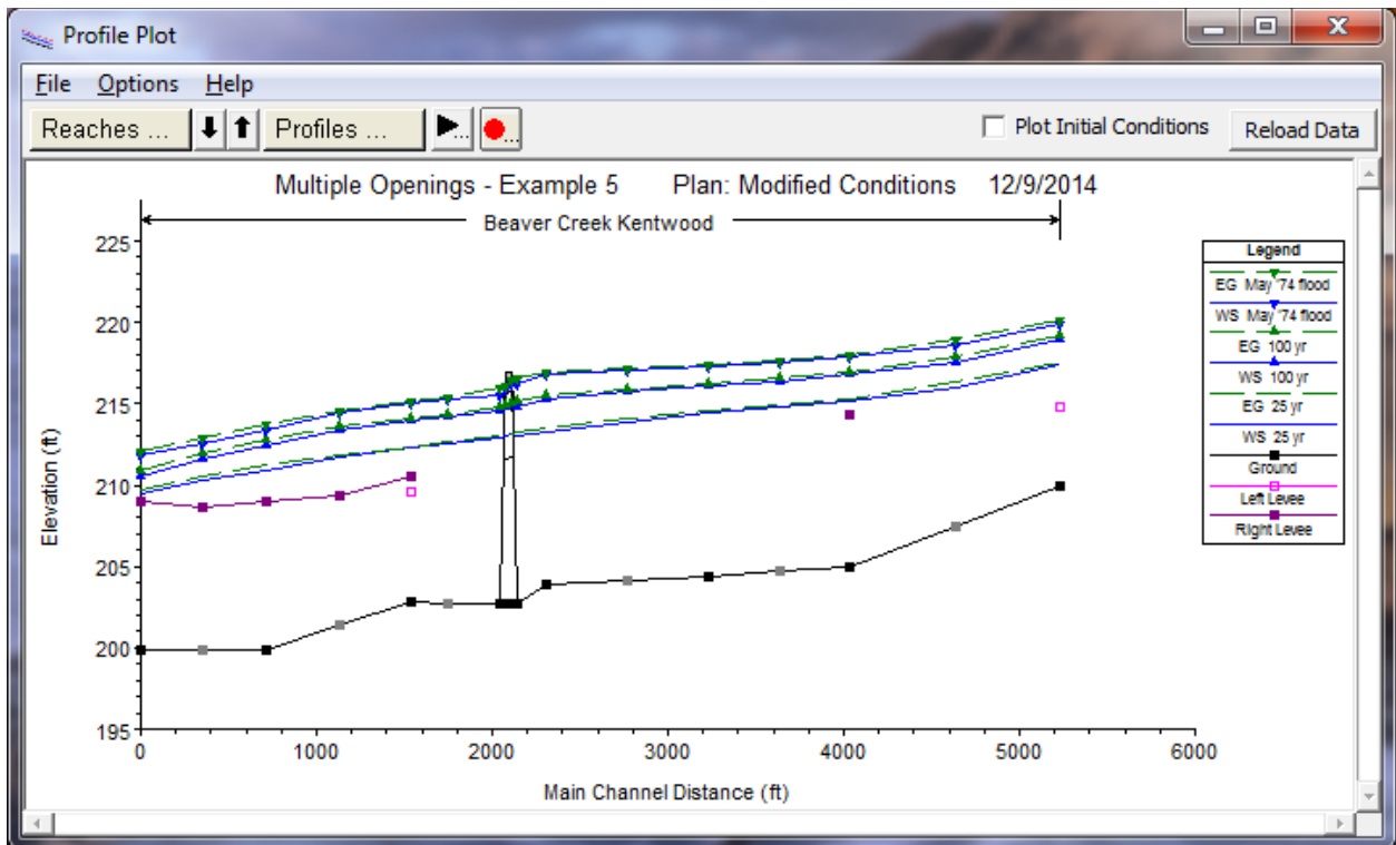
Figure 5-9: Water Surface Profiles for Modified Conditions Plan
