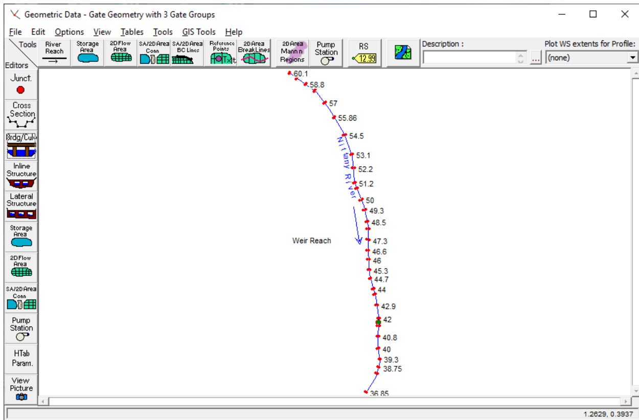
Figure 12-1: River System Schematic for Nittany River
