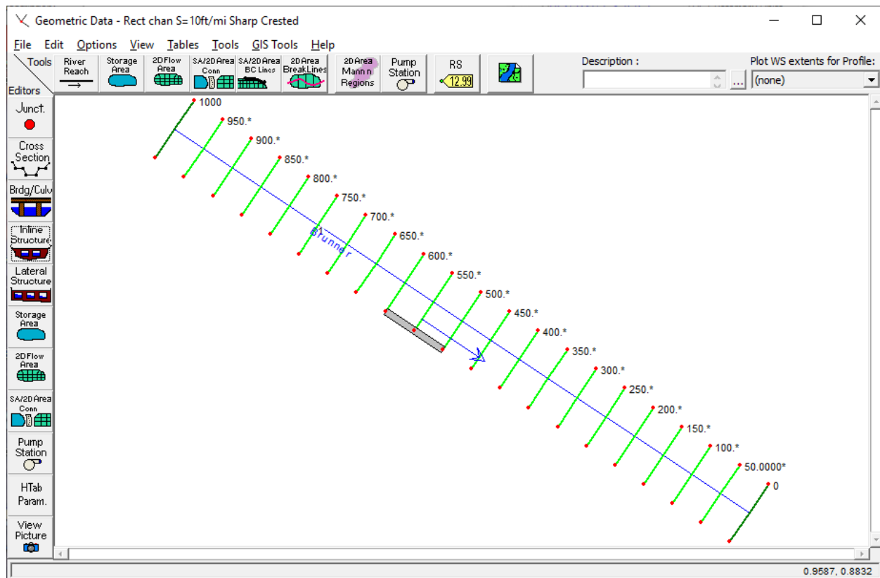
Figure 20-1. River System Schematic for Brunner River
