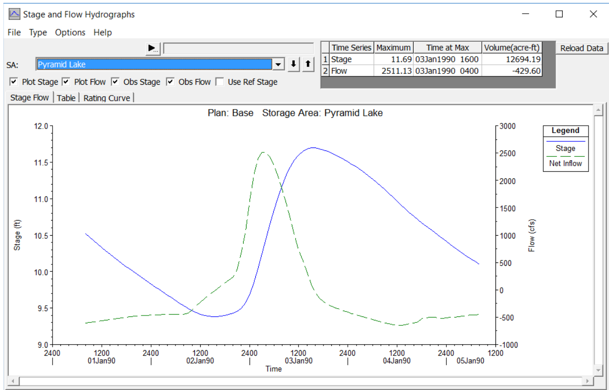
Figure 17-24: Stage and Flow Hydrograph for Pyramid Lake
