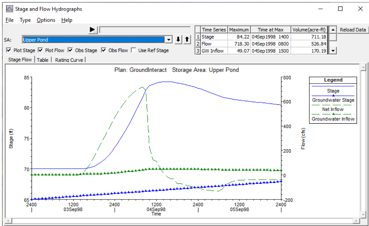
Figure 22-15. Stage and Flow Hydrograph for Upper Pond
