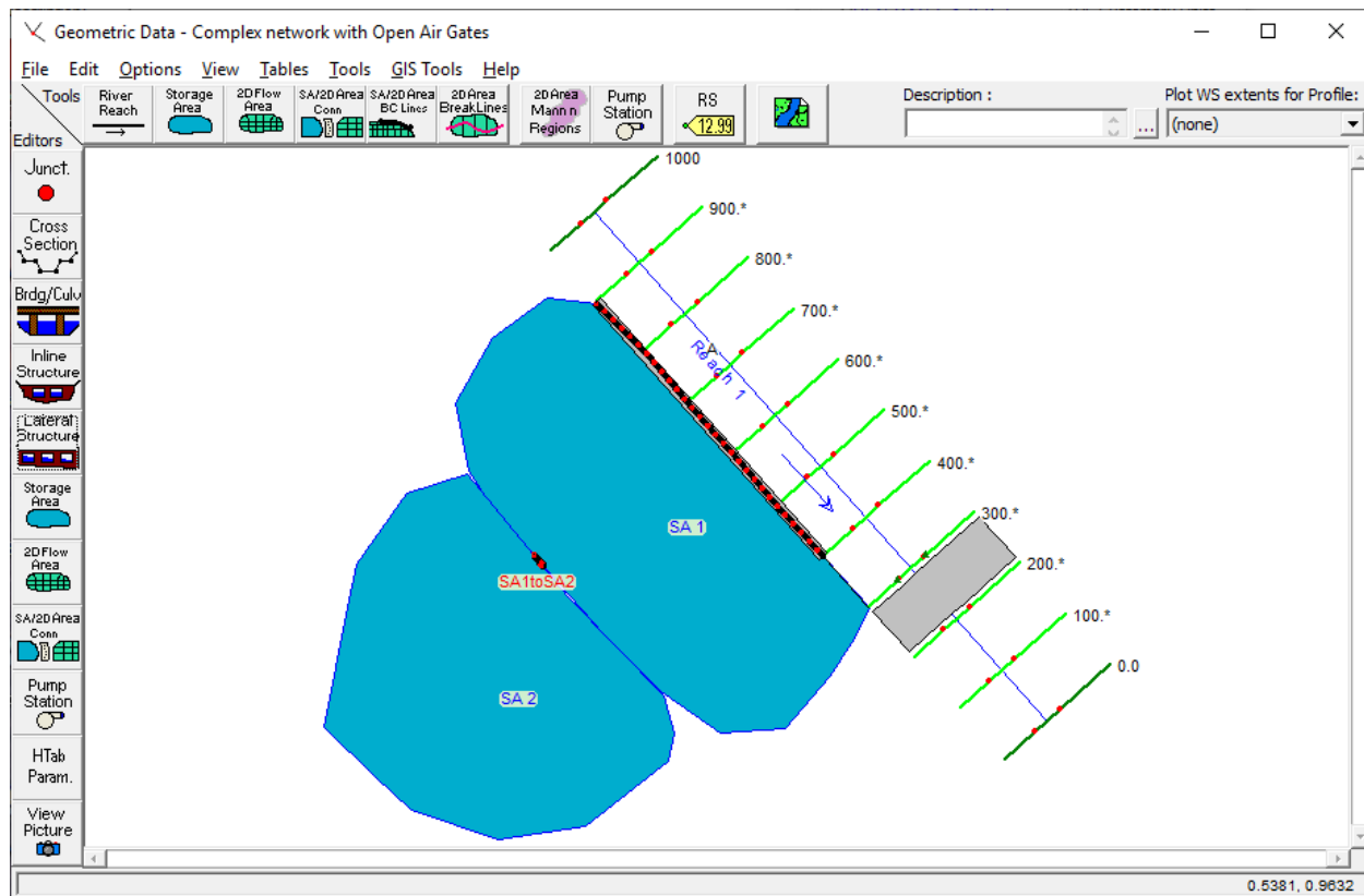
Figure 21-1. River System Schematic for Marston Creek with Storage Areas
