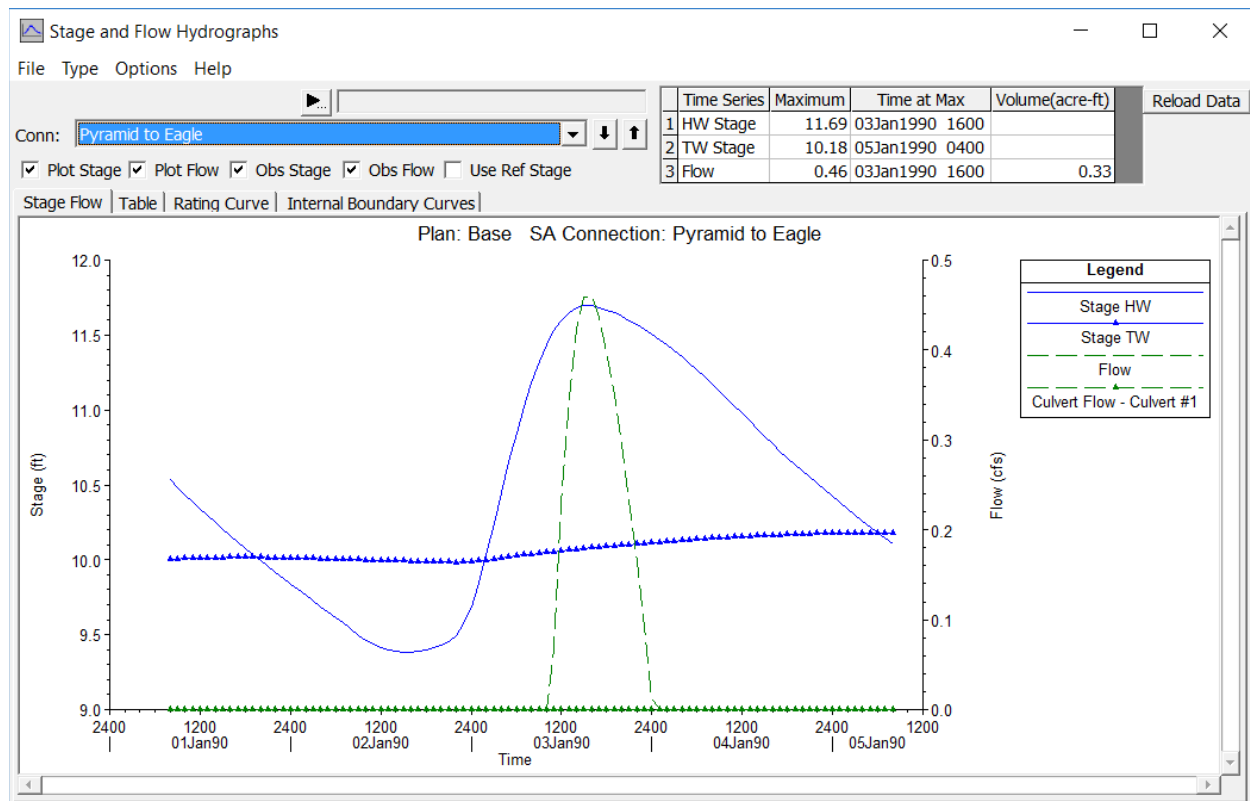
Figure 17-25: Stage and Flow Hydrograph for Hydraulic Connection – Pyramid to Eagle
