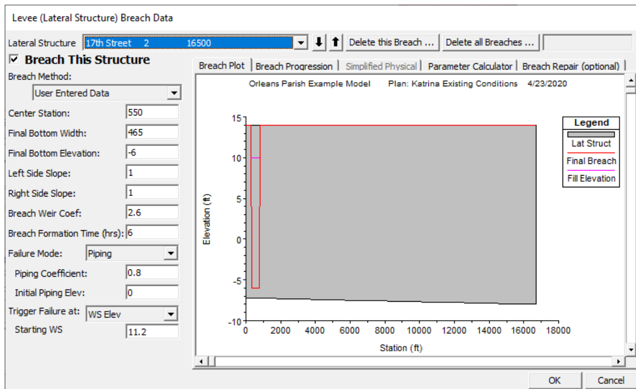
Figure 23-11. Levee (Lateral Structure) Breach Data Editor
