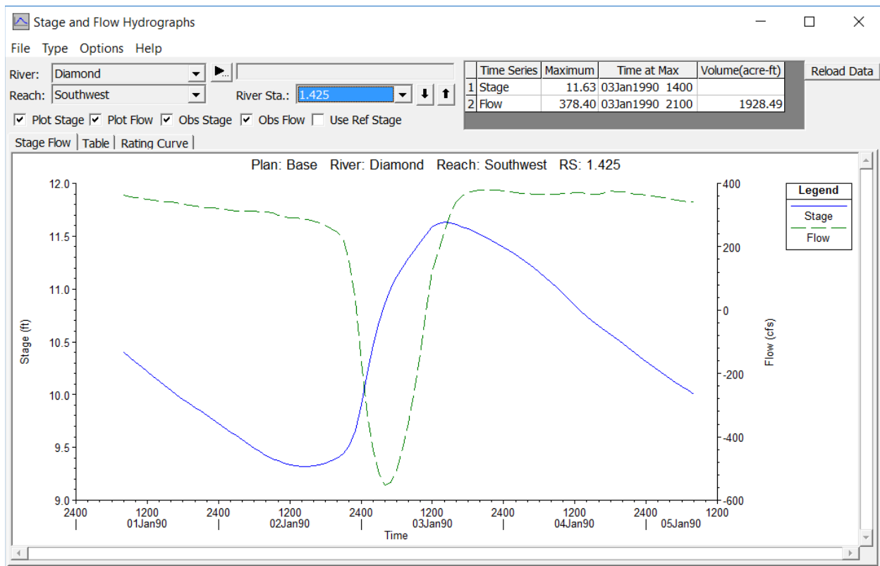
Figure 17-22: Stage and Flow Hydrograph for Southwest Reach
