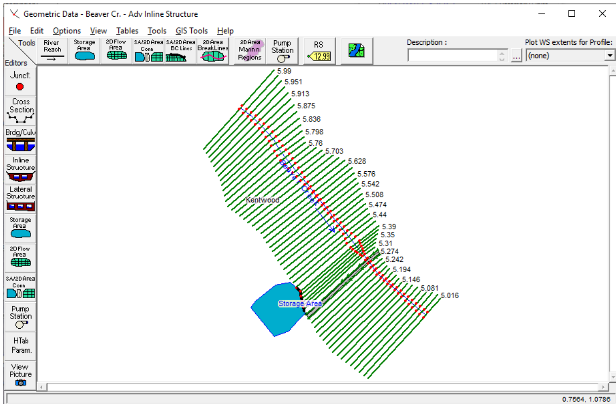
Figure 18-1. River System Schematic for Beaver Creek
