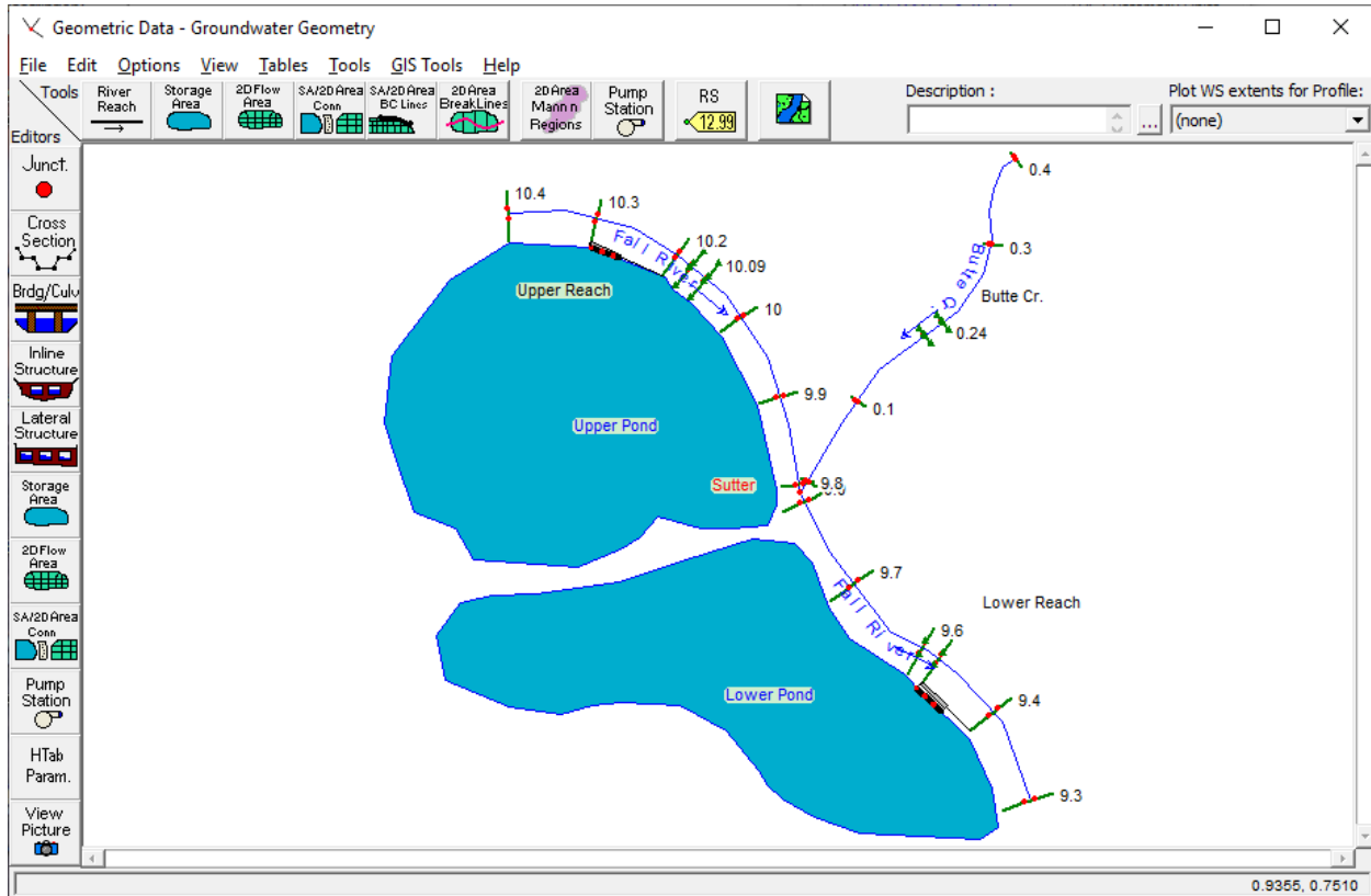
Figure 22-1. River System Schematic
