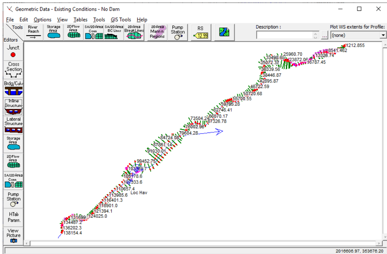
Figure 19-1. River System Schematic for Bald Eagle River
