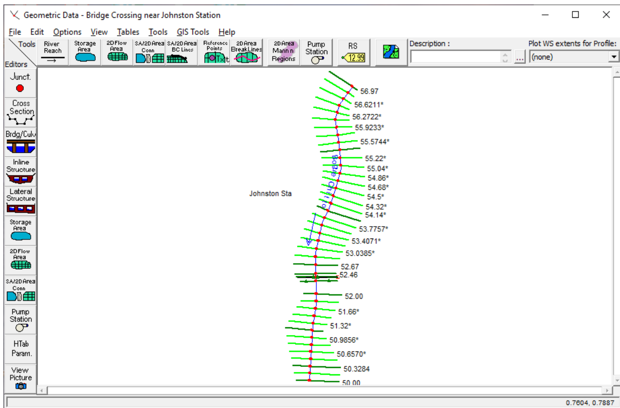
Figure 13-1: River System Schematic
