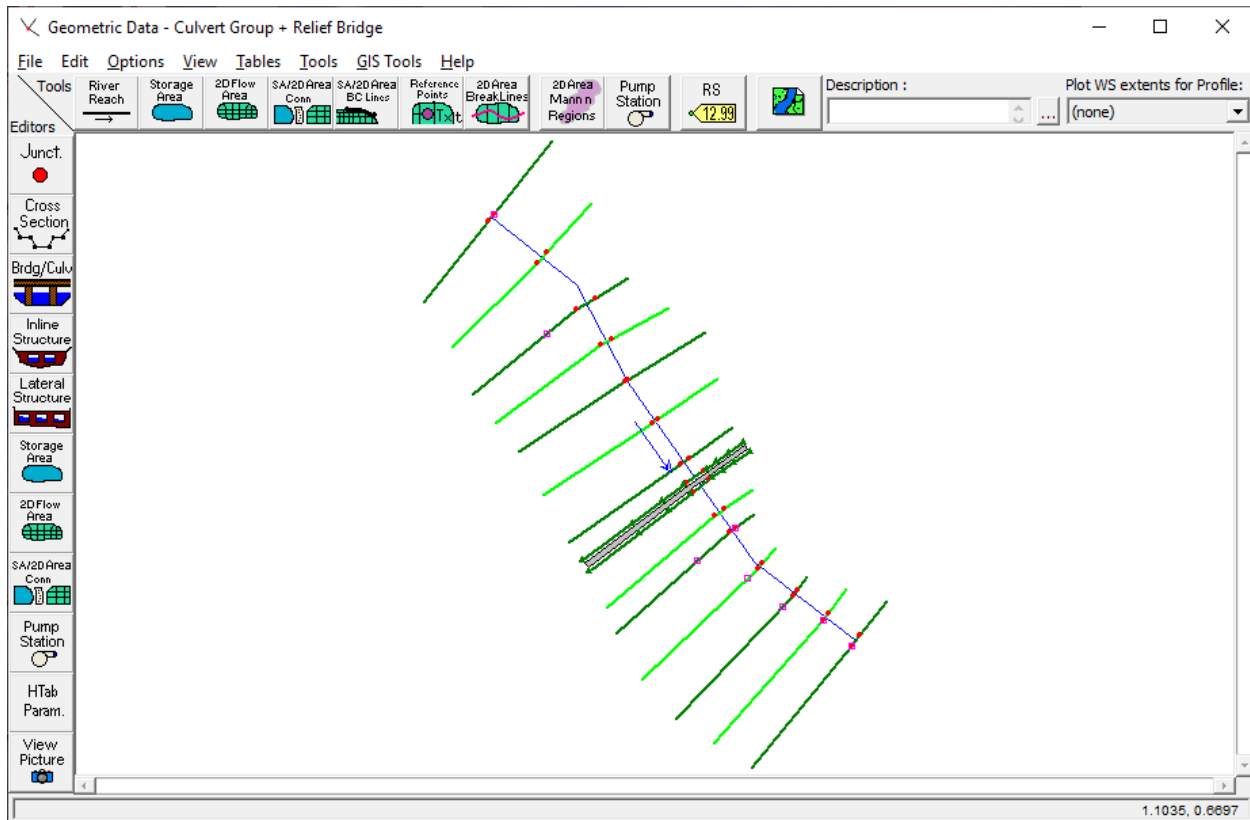
Figure 5-1: River System Schematic
