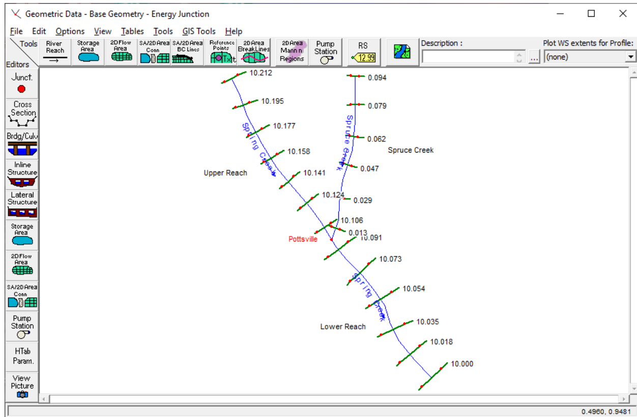
Figure 10-1: River System Schematic
