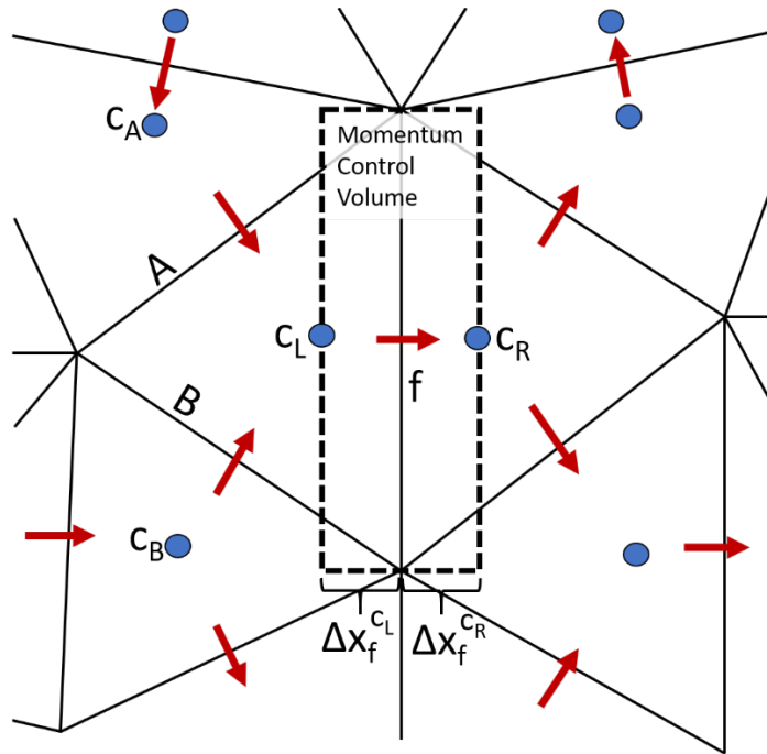
Figure 2-19. Control Volume for Conservation of Momentum (from Kramer and Stelling, 2008)
