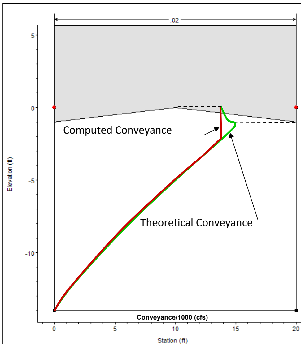
Figure 4-16. Theoretical and Computed Conveyance
