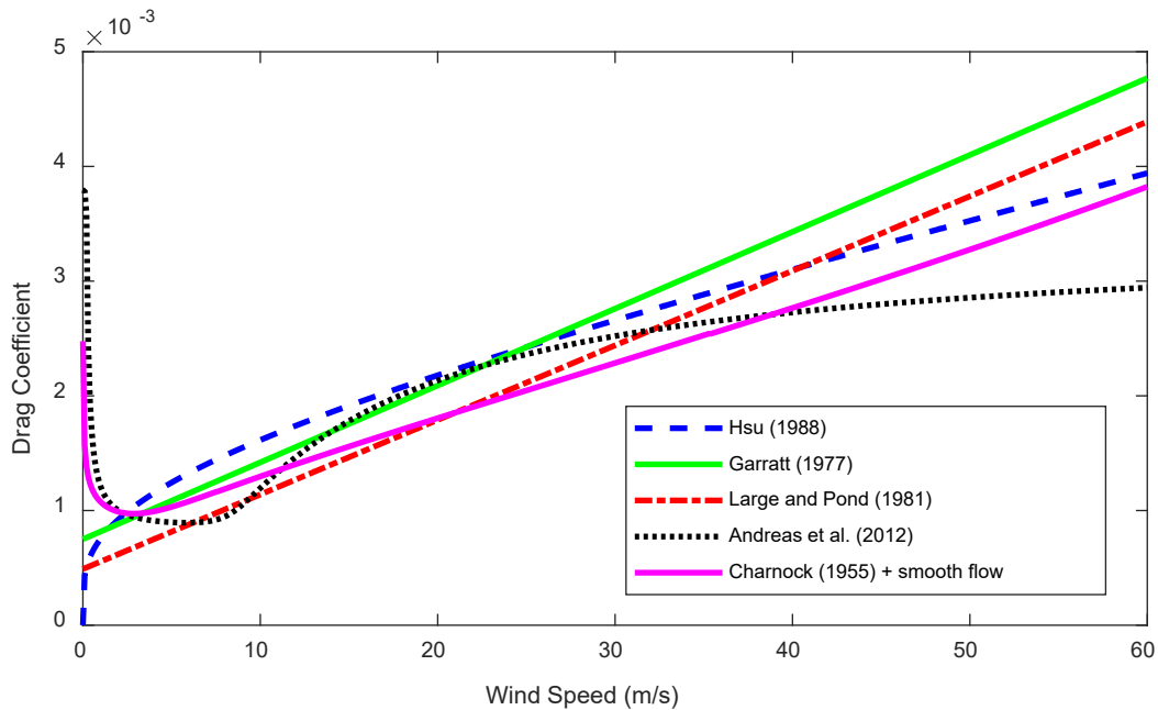
Figure 2-17. Wind drag coefficient.
