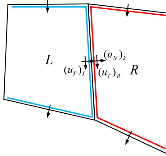
Figure 2-20. Double-C stencil used for computing the face tangential velocity.
