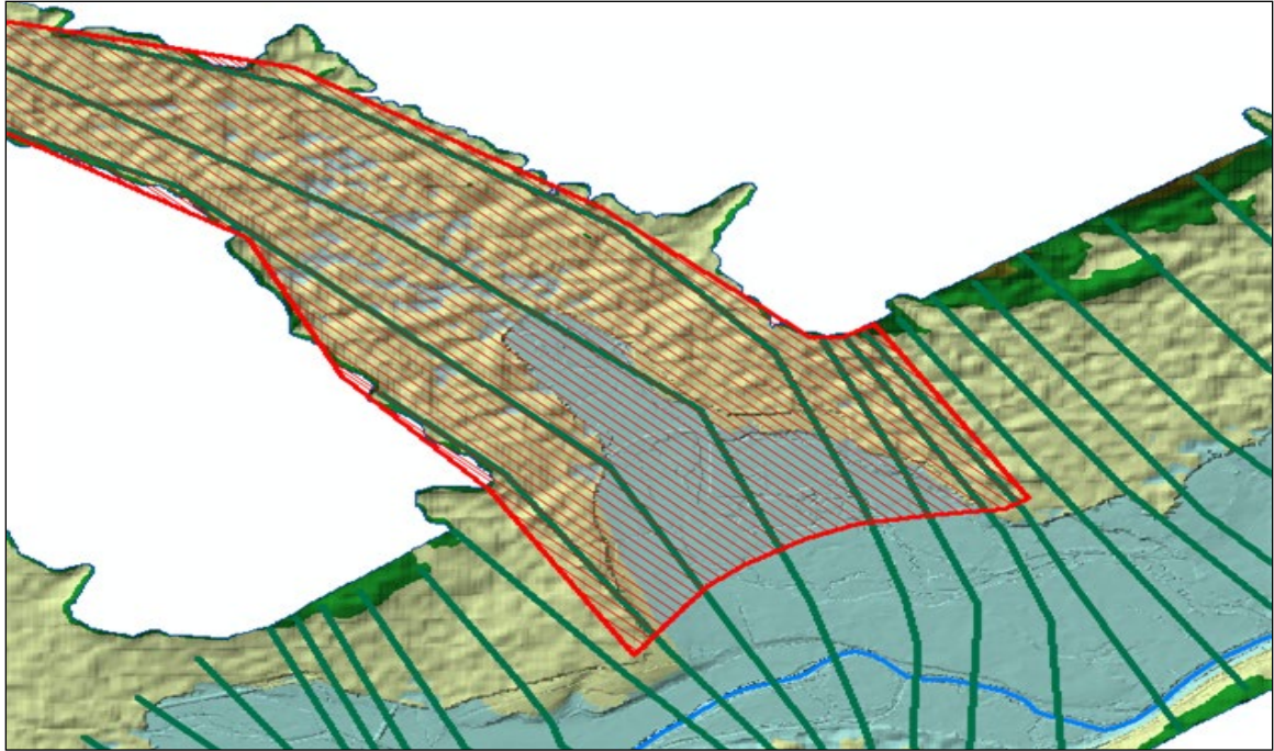
Figure 13-19. Tributary storage modeled as cross section ineffective flow areas.
