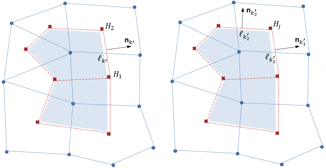
Figure 2-19. Cell and Dual Cell Finite Volume Formulation
