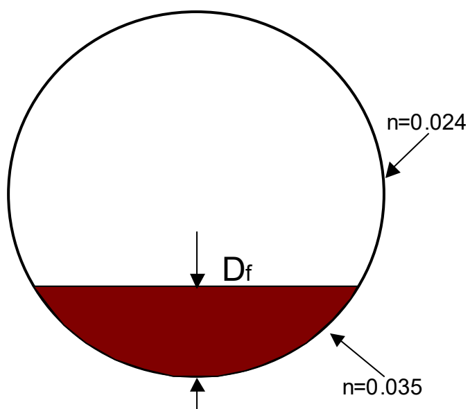
Figure 6-11 Partially Filled or Buried Culverts
